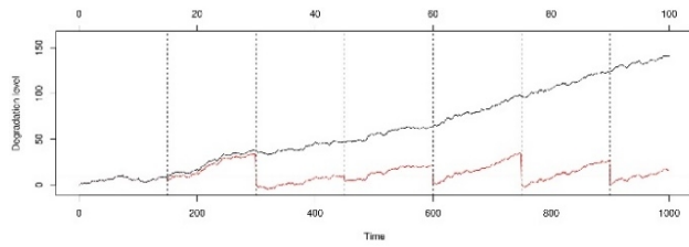
Figure 4. \text{ARD}(\infty) of the second component with \rho = 0.5 .
