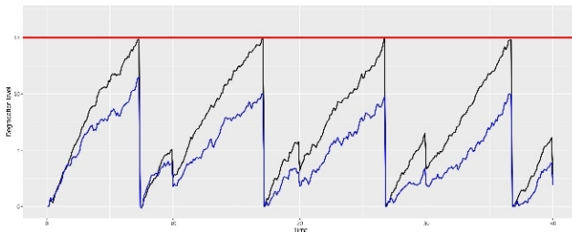
Figure 10. Realization of the ARD maintenance model.
