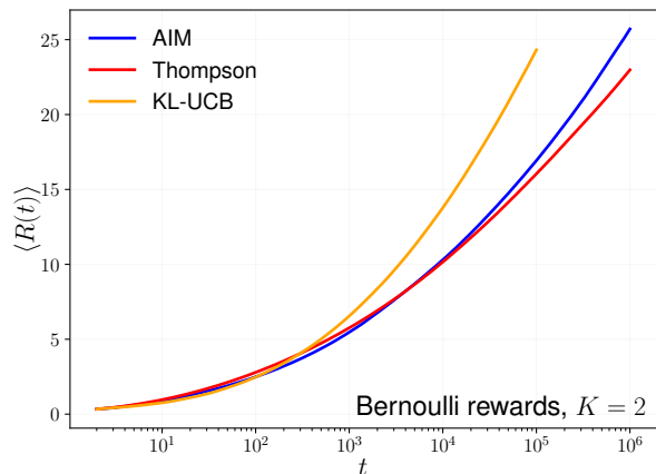
Figure 3: Evolution of the Bayesian regret for 2-armed bandit with Bernoulli rewards under a uniform mean prior. The regret is averaged over more than 10^5 runs.
