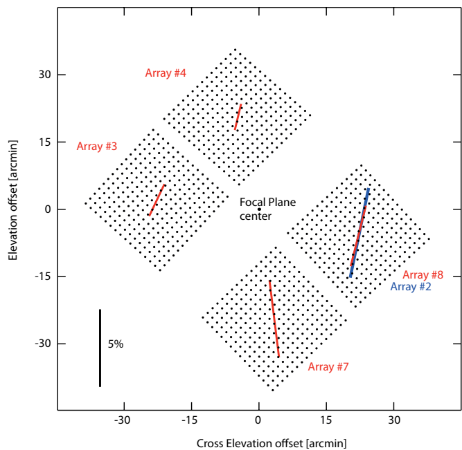
Fig. 6: Distribution of the leakage polarization direction and intensity across the PILOT focal plane. The focal plane is shown in instrument coordinates, with elevation corresponding to the vertical direction, in offsets from the focal plane center. The circles show the positions of individual pixels of the TRANS arrays. The labels give the name of each operational array in red and blue for the REFLEX and TRANS focal plane respectively. The lines show the direction and amplitude of the intensity to the polarization leakage as measured on Jupiter for each array independently, in red and blue for the REFLEX and TRANS arrays respectively. The scale on the bottom left shows 5%.
