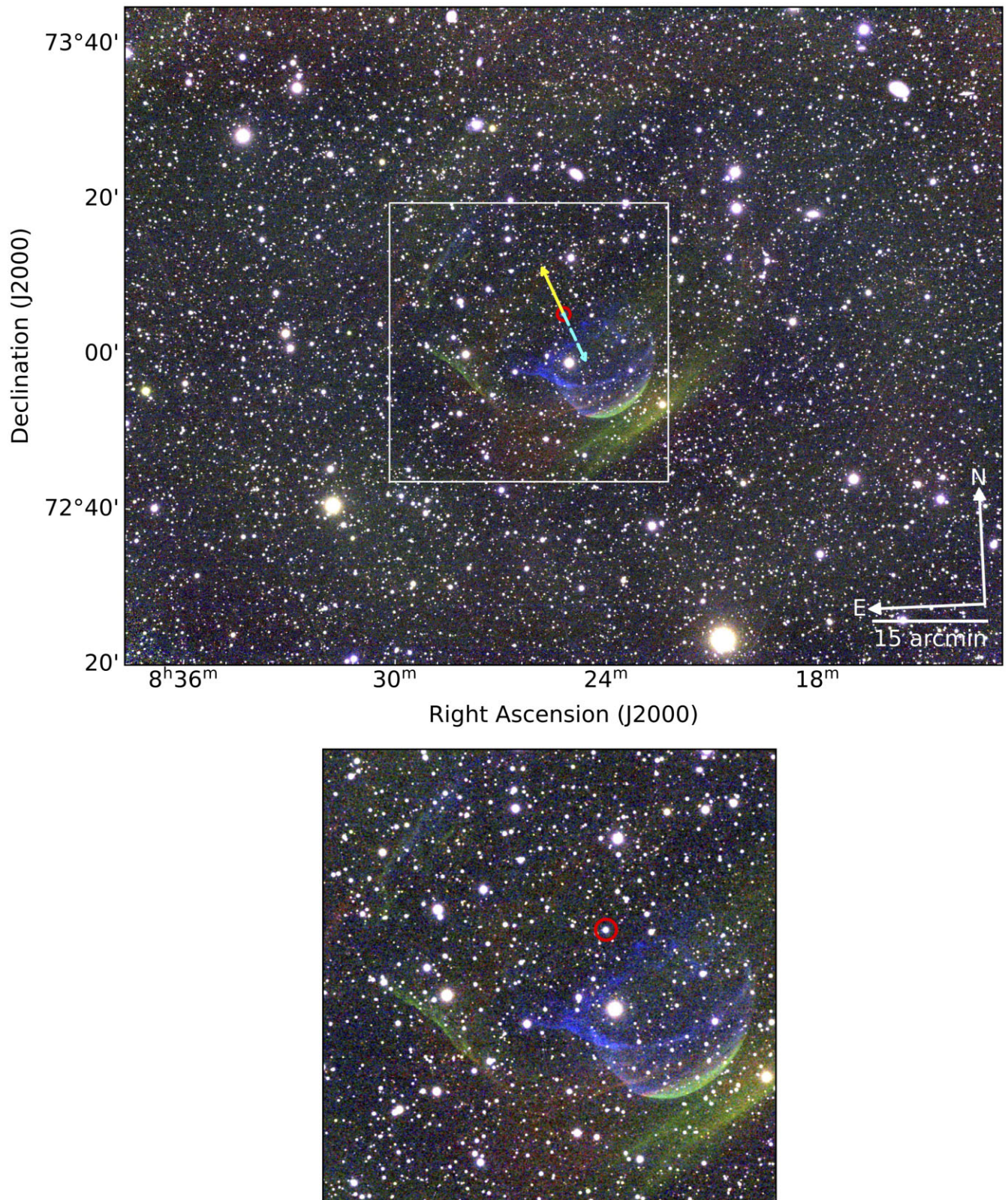
Figure 2. Top: Area surrounding Z Cam in Condor [S II], H \alpha + [N II], and [O III] in red, green, and blue, respectively. Z Cam is circled in red. The images have been smoothed via a Gaussian kernel ( \sigma = 2.5 pixels) and are displayed with asinh scaling. The current direction of motion (from Gaia , Bailer-Jones et al. 2021) of Z Cam is shown with a dashed cyan arrow, and the solid yellow arrow points to the location of Z Cam 20 000 yr ago. Bottom: The area of the region containing the SW arc, SE linear feature, and NE linear feature (denoted by the white box) is shown enlarged.
