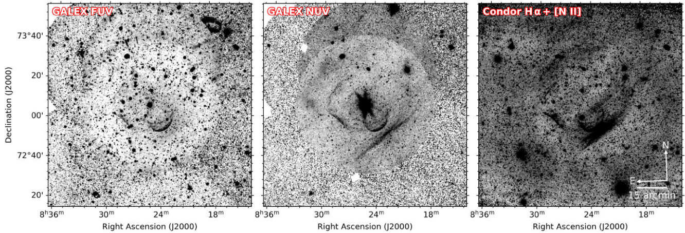
Figure 5. Comparison of GALEX FUV, GALEX NUV, and Condor H \alpha + [N II] images in the region surrounding Z Cam. The Condor image has been downsampled by a factor of 16 with averaged pixel blocks and is displayed inverted with linear scaling.
