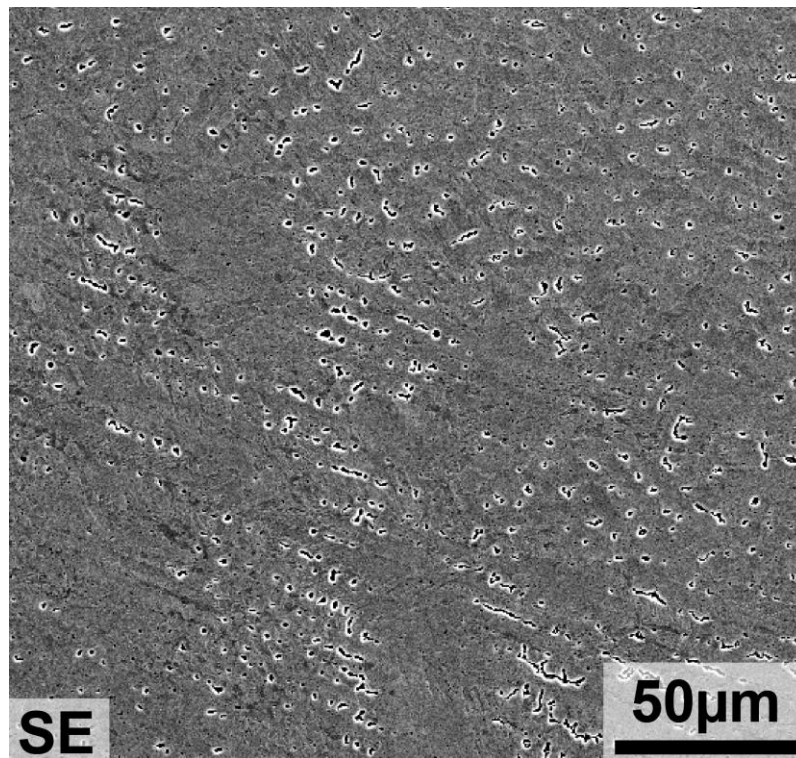
Fig. S1 Secondary electron (SE) micrograph acquired at a Ti composition of 6at% occurring in microstructure regime number 1 at low Ti content. This micrograph shows that at such Ti compositions a small amount of Laves phase occurs. The Laves phase is indicated by the small dark regions surrounded by a bright ring. The dark regions is due to the fact that the Ti rich Laves phase is preferentially etched out by Nital. The surrounding bright outlines are due to the so called “edge effect” (i.e. edges emitting high amounts of electrons) in SEM.
