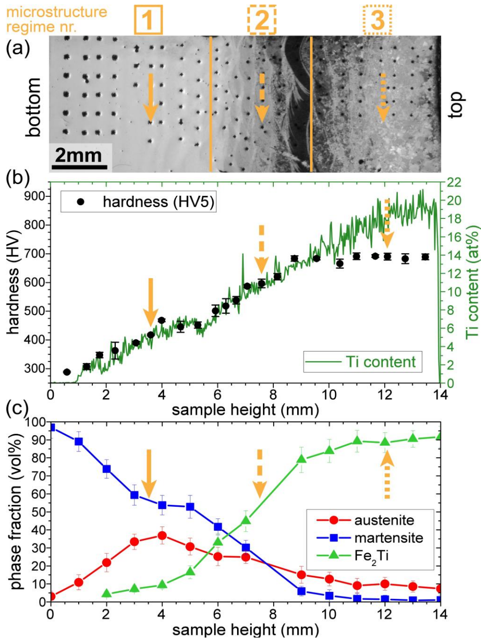
Fig. 1 Overview of the Ti graded specimen produced by DED for this study. (a) is a light optical micrograph after Nital etching. The different microstructure regimes that occur at low, intermediate and high Ti contents are separated by vertical orange lines and indicated by numbers. The regular array of dark spots corresponds to the indents from hardness measurements. Orange arrows in this figure mark the locations (i.e. corresponding Ti compositions) for the in-depth microstructure characterization described in section 3.2. (b) shows the Ti composition from SEM-EDS quantification as a function of the sample height overlaid with hardness. The increase in Ti content along the sample build height is accompanied by a steep increase in hardness up to 14 at% Ti where a plateau in hardness at around 700 HV is reached. (c) depicts the phase
