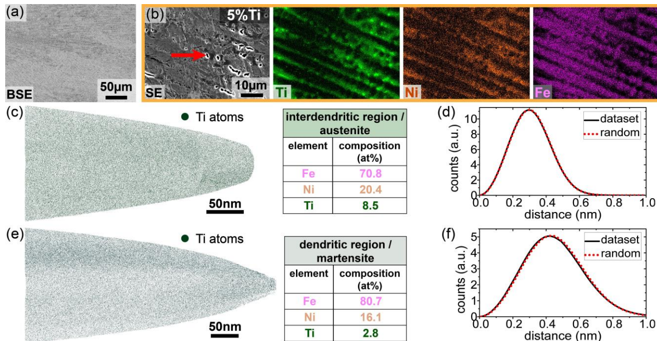
Fig. 2 In-depth characterization of the microstructure at 5 at% Ti composition representative for microstructure regime number 1 at low Ti content. (a) depicts a backscatter electron (BSE) micrograph at low magnification demonstrating microstructure homogeneity at large length scale. The SEM-EDS mapping in (b) visualizes the dendritic solidification structure with Ni and Ti being enriched at the interdendritic regions. A small amount of Laves phase can be seen in the SE micrograph. Because the Ti rich Laves phase is preferentially etched by Nital, it is indicated by dark regions, surrounded by bright outlines which are due to the so called “edge effect” (i.e. edges emitting high amounts of secondary electrons) in SEM. One of the Laves phase particles is marked by a red arrow. (c) and (d) show APT results from an interdendritic region, (e) and (f) from a dendritic region. Atom maps in (c) and (e) show Ti atoms in a thin slice of 5 nm thickness through the APT reconstruction. The nearest neighbor distributions in (d) and (f) demonstrate a random distribution of Ti.
