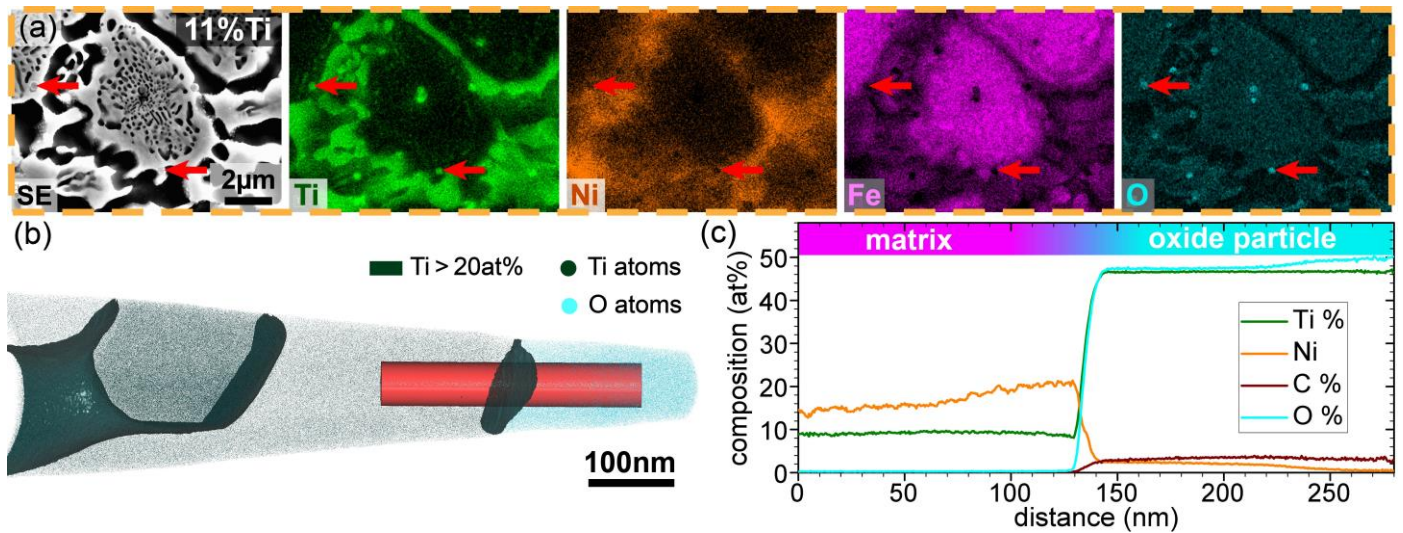
Fig. S4 In-depth characterization of the microstructure at 11 at% Ti composition representative for microstructure regime number 2 at intermediate Ti content. Additionally, to the elemental mappings shown in Fig. 3 in the main section, the O mapping is shown in (a) here to demonstrate the distribution of fine Ti-oxide particles. (b) and (c) depict APT results from this regime. The atom map in (b) features 0.5% of the Ti atoms in green and 3% of the O atoms in blue in the reconstructed volume. Regions with Ti contents higher 20 at% are highlighted by a green iso-composition surface. On the left (bottom of the measured APT tip) the iso-composition surface marks a Laves phase, on the right (top of the measured APT tip) it marks a Ti-oxide particle. Due to the O ions, this oxide particle appears blue in the figure. A composition profile along the red cylinder is shown in (c). The oxide particle contains around 48-49at% Ti, the same amount of O and 3-4at% C.
