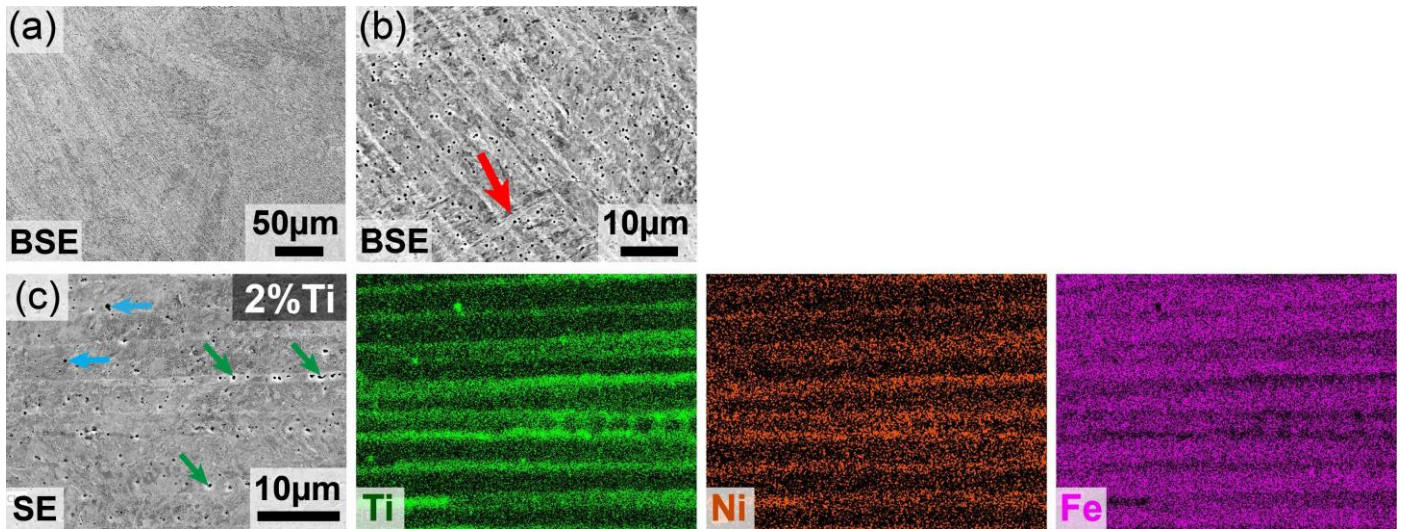
Fig. S2 In-depth characterization of the microstructure at 2 at% Ti composition occurring in microstructure regime number 1 at low Ti content. (a) and (b) present backscatter electron (BSE) micrographs, (c) a secondary electron (SE) micrograph together with the corresponding SEM-EDS mapping. A cellular dendritic solidification structure with Ti and Ni microsegregation at interdendritic regions can be observed. A martensitic microstructure is overlaid onto this solidification. At interdendritic regions with very strong segregation austenite can be stabilized. Martensite laths crossing multiple dendrites/cells are marked by a red arrow in (b). Some of the dark spots seen in the secondary electron micrograph in (c) are small Lave phase particles which are etched out and show a characteristic bright rim as a result of the so-called edge effect. Some of the dark spots are oxide particles which appear more resistant to etching. Some examples of oxide particles are marked by blue arrows, some Laves phase particles by green arrows.
