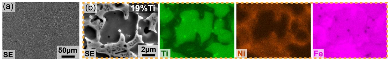
Fig. 4 In-depth characterization of the microstructure at 19 at% Ti composition representative for microstructure regime number 3 at high Ti content. (a) depicts a secondary electron (SE) micrograph at low magnification demonstrating microstructure homogeneity at large length scale. The SEM-EDS mapping in (b) visualizes the eutectic solidification structure occurring at this Ti composition. Ni and Ti are enriched at different regions because here a different primary phase forms compared to the eutectic microstructure at intermediate Ti compositions.
