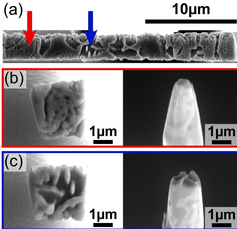
Fig. S3 SEM pictures during FIB preparation. (a) shows an electron micrograph of the piece lifted out from the DED sample from which the individual pieces are chopped off that are then prepared into APT specimen by annular FIB milling. (b) and (c) show the top of such pieces on the left as well as a side view of the specimen during annular FIB milling.
