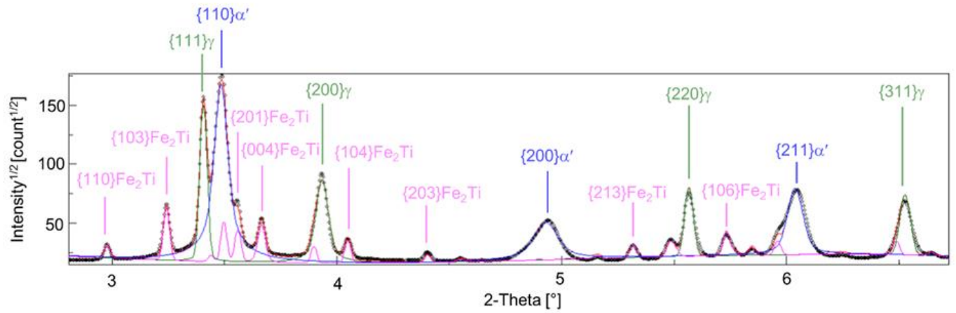
Fig. S5 HEXRD diffractogram obtained from Rietveld analysis (sample height= 7mm). The experimental diffractogram obtained by HEXRD is represented by black dots while those depicted in green, pink and blue, represent those obtained by phase analysis of the austenite ( \gamma ), Fe 2 Ti and martensite ( \alpha' ), respectively, using the Rietveld method (see methodology section).
