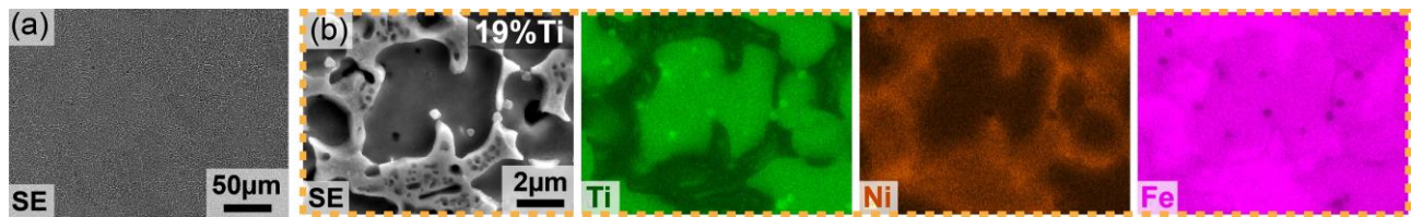
Fig. 4 In-depth characterization of the microstructure at 19 at% Ti composition representative for microstructure regime number 3 at high Ti content. (a) depicts a secondary electron (SE) micrograph at low magnification demonstrating microstructure homogeneity at large length scale. The SEM-EDS mapping in (b) visualizes the eutectic solidification structure occurring at this Ti composition. Ni and Ti are enriched at different regions because here a different primary phase forms compared to the eutectic microstructure at intermediate Ti compositions.
