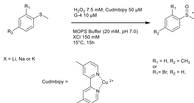
Scheme 2. Sulfoxidation of thioanisole derivatives. G-4 = HT21, tetramolecular G-4, mimic 1a-h or 2 .
