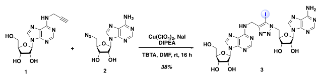
Scheme 1. Synthesis of 5-iodo-triazole 3 .
