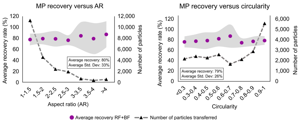
Fig. 6 The diagrams plot average recovery of FMPs and SMPs combined, versus AR (left), and circularity (right). The total number of transferred particles within the specified ranges is marked by black triangles. Average recovery based on AR shows stability around the overall average recovery of 80% at AR < 3. Above this threshold the number of transferred particles becomes statistically insignificant and std. dev. increases significantly. RR of MPs of both high and low circularity showed reasonable stability around the overall average RR of 79%, yet at AR 0.6–0.7, standard deviation increased significantly. Note that high std. dev. coincides with low number of transferred particles
