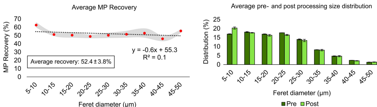
Fig. 8 The diagrams display (left) average RR of FMP fragments at a spatial resolution on the order of 5 \mu\text{m} . Average recovery was estimated at 52.4 \pm 3.8\% and was largely independent of particle size, with the exception of a noticeable higher RR in the 5–10 \mu\text{m} range. This augmented recovery resulted in a relative concentration enhancement of the smallest size fraction depicted in the histogram (right) displaying average MP size distribution, pre- and post-sample processing. This concentration enhancement may be the result of particle agglomeration and/or particle breakup during sample manipulation
