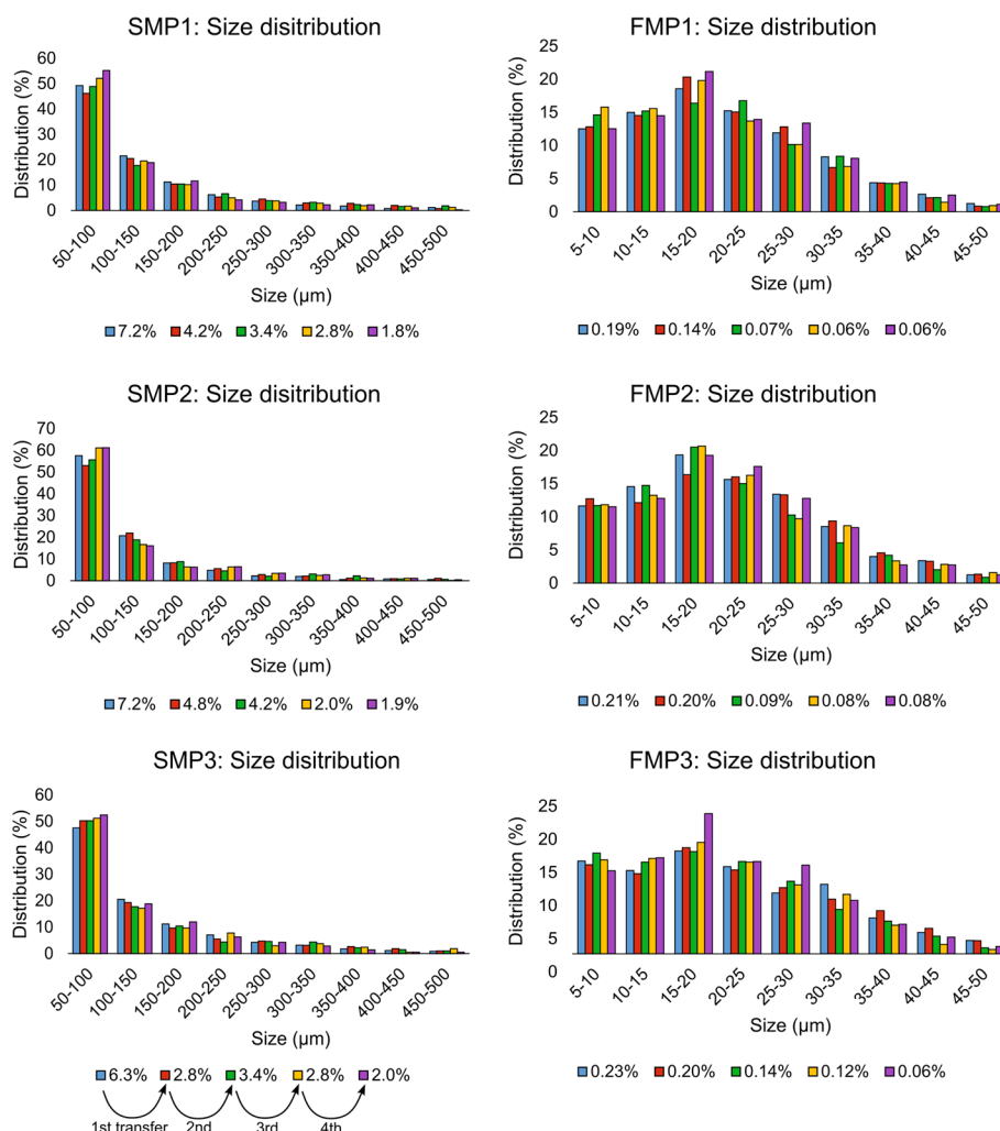
Fig. 9 Histograms visualizing the MP distribution within specified size groups, following each individual transfer. legends refer to the filter area occupied by particles (A%). Size distribution of MPs remains relatively stable following four successive transfers, yet SMPs display an increase in the smallest size fraction with decreasing A%. As a general trend, this tendency was not observed in FMPs and may therefore be linked to excessive A%, leading to increased probability of particle agglomeration and concealment
