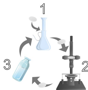
Fig. 1 (1) Using a glass vacuum filtration device, particles were filtered onto a 25 mm, 0.65 µm PVDF filter membrane. (2) Photomicrographs were captured under darkfield illumination in order to determine the quantity and morphological parameters of the transferred MPs. (3) All particles on the examined filter were subsequently flushed with ultrapure Milli-Q water, into a 40 mL glass bottle. The content of the bottle was then poured, flushed and filtered onto another PVDF filter membrane. This process was repeated four times for each sample
