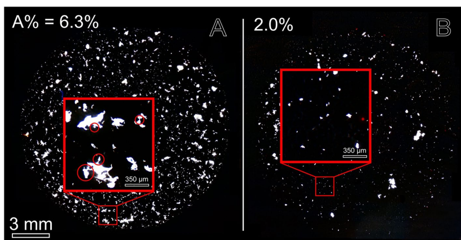
Fig. 10 Photomicrographs visualizing the difference between the potential of particle overlap, concealment and agglomeration when (A) A% = 6.3% versus (B) A% = 2.0%. Red rings indicate episodes where smaller particles have agglomerated onto larger particles, thereby causing underestimation of the number of smaller MPs. When the filter is less charged, this is probabilistically less likely to occur
