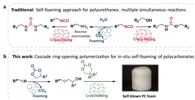
Scheme 1. General comparison of the self-foaming approaches for PUs and PCs, highlighting the similarities between the gelation and foaming processes. (a) Overview of the traditional self-foaming method for PUs to execute multiple, simultaneous reactions. (b) General description of a decarboxylative cascade ring-opening polymerization for the preparation of self-blown PC foams facilitated by an in situ formed reactive \beta -hydroxythioether intermediate upon the S-alkylation by the cyclic carbonate.
