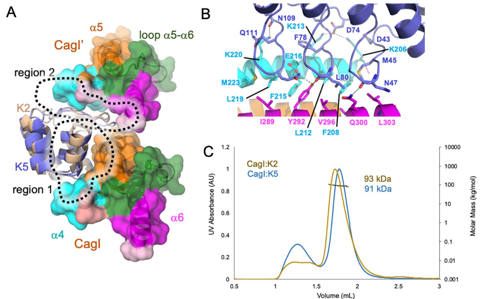
Fig 4. Structural basis for higher affinity of DARPin K2 on CagI. A) Overview of the structures of the CagI:K2 and CagI:K5 complexes interfaces. The two DARPin structures K2 (wheat) and K5 (blue) have been superimposed and are depicted as cartoons. The CagI molecule and symmetry related CagI' are displayed as cartoons and surfaces are coloured as in Fig 3. For clarity, only CagI molecules from the CagI:K2 complex are displayed. B) detailed view of region 2 interactions between DARPin K5 loop residues and CagI α4 and α6 with involved side chains displayed as ball and sticks with atoms coloured as follows: nitrogen in blue, oxygen in red, carbon as in A). Dashed lines indicate hydrogen bonds. C) SEC-MALS measurements of the CagI:K2 and CagI:K5 purified complexes.
