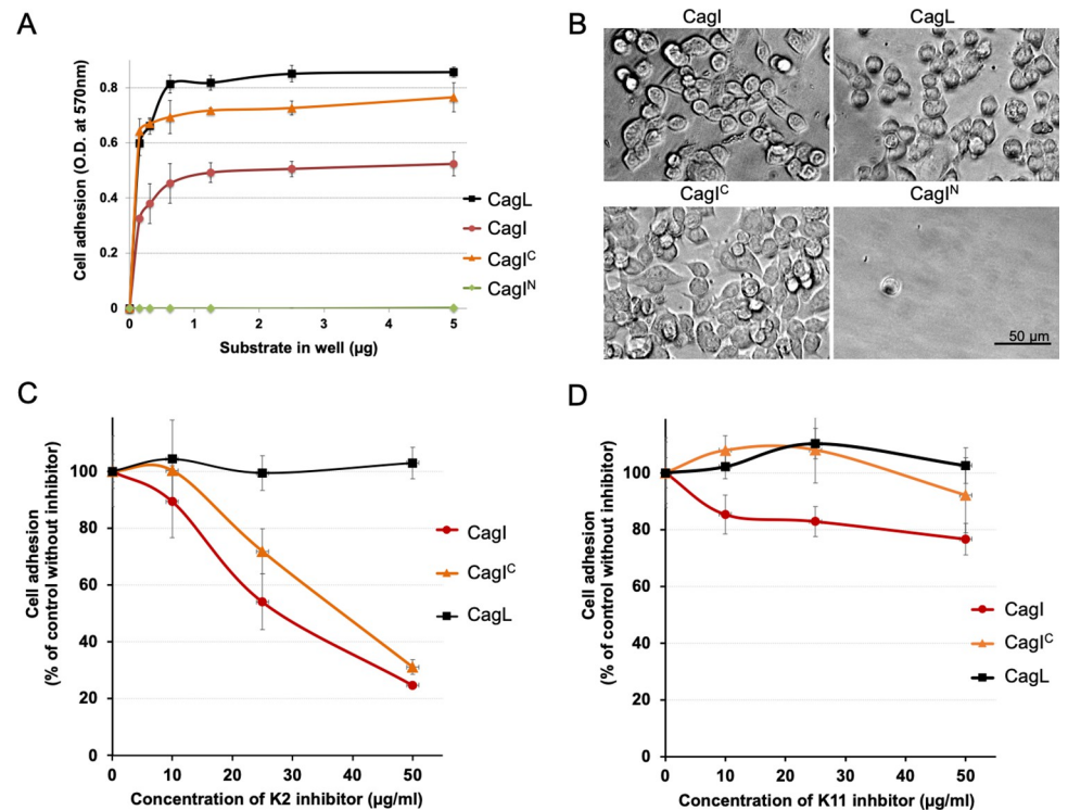
Fig 6. Cell binding and spreading to cagT4SS proteins and domains. A) Dose-dependent AGS cell adhesion to CagL, CagI, CagI C and CagI N . Multiwell plates were coated with different amounts of the proteins as indicated on the Figure. Each assay point was derived from triplicate measurements. B) Representative images of adhered AGS cells on well-surfaces coated with 0.15 μg of indicated proteins. C) Effect of DARPin K2 or D) K11 on adhesion of AGS cells to CagL, CagI, CagI C . Multiwell plates were coated with 4 μg of each protein. After saturation with 1% BSA, the wells were incubated with 50 μL of the indicated concentration of K2 or K11 for 1 h at room temperature, and the cells were seeded in the presence of the inhibitor. The extent of adhesion was measured as previously described and expressed as percentage of adhesion to each protein in the absence of the inhibitor. Each assay point was derived from triplicate measurements.
