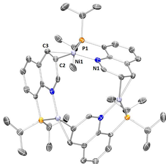
Figure 5: Ortep plot of [NiL] 3 with thermal ellipsoids (drawn at the 50% probability level). The H atoms were omitted for clarity. Selected bond lengths [Å] and angles [°]: Ni1-N1 1.960(7), Ni1-P1 2.150(3), Ni1-C2 1.985(9), Ni1-C3 1.981(8), C2-C3 1.459(12), N1-Fe1-P1 88.7(2), N1-Ni1-C2 115.5(3), C3-Ni1-C2 43.2(3), C3-Ni1-P1 113.0(3)
