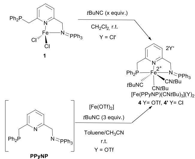
Scheme 2: Access to [Fe(PPyNP)(CNTtBu) 3 ] 2+ complexes
