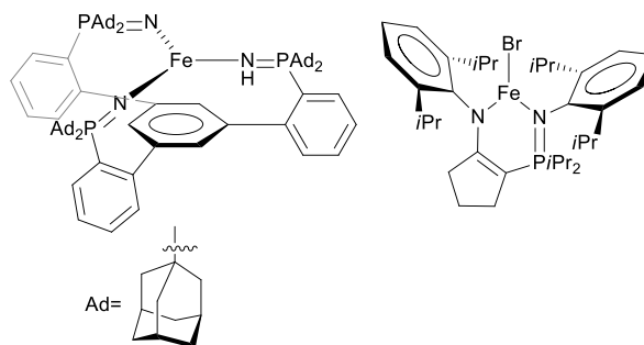
Figure 2: Fe II iminophosphorane complexes for small molecules activation
