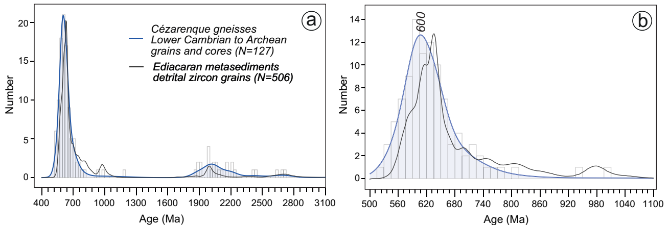
Fig. 10. Histograms and Kernel Density Estimates (plotted with an adaptive bandwidth) showing the U–Pb date distribution of older-than-Lower Cambrian zircon grains, rims, and cores from the Cézarenque–Joyeuse gneisses. Only concordant ^{206}\text{Pb}/^{238}\text{U} dates (if < 1.2 Ga) and concordant to slightly discordant ( ^{206}\text{Pb}/^{238}\text{U} date/ ^{207}\text{Pb}/^{206}\text{Pb} date > 92\% , if > 1.2 Ga) were considered. The data are compared to the U–Pb date distribution of Ediacaran metasediments from the Cévennes parautochthon of the eastern Massif Central, also represented as Kernel Density Estimates (Chelle-Michou et al. , 2017; Couzinié et al. , 2019).
