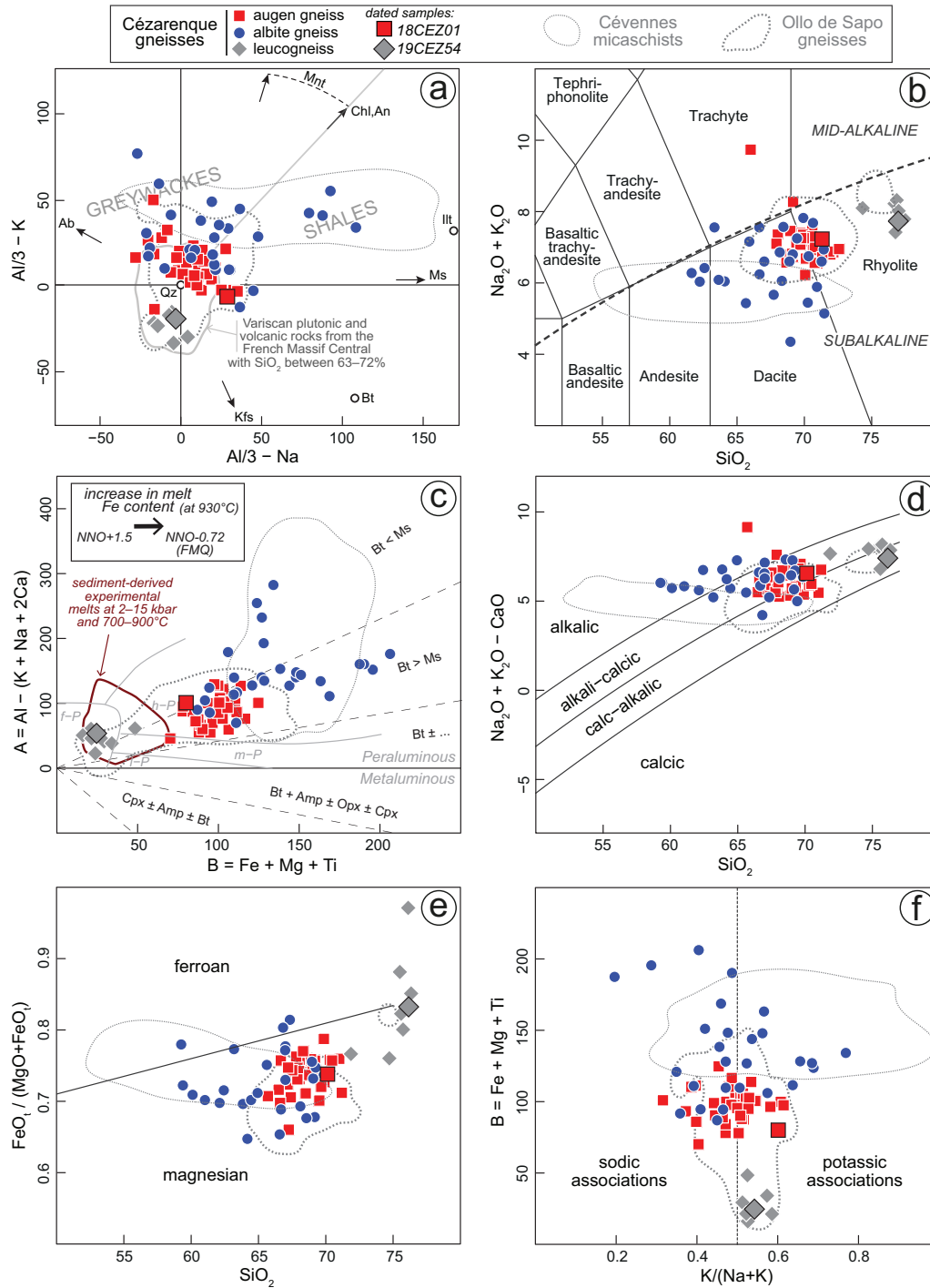
Fig. 6. Whole-rock geochemistry of the Cézarenque–Joyeuse gneisses. (a) Al/3-K vs. Al/3-Na cationic diagram of de La Roche (1968) aiming at discriminating meta-igneous from metasedimentary rocks. (b) Total alkali vs. silica classification diagram of Le Bas et al. (1986) . The dashed line is the subalkaline–mid-alkaline boundary following Rittman (1957) . (c) B–A cationic classification diagram of Debon and Le Fort (1988) with the subdivisions of Villaseca et al. (1998) . (d) SiO 2 vs. Na 2 O + K 2 O – CaO and (e) SiO 2 vs. FeO t /(FeO t + MgO) (in wt.%) diagrams of Frost et al. (2001) . (f) K/(K + Na) vs. B. cationic classification diagram of Debon and Le Fort (1988) . The dotted lines represent the contours encompassing 85% of the data for the following distributions: Variscan plutonic and volcanic rocks from the French Massif Central with SiO 2 between 63–72% ( n = 1350, Moyen et al., 2017 ), the Ollo de Sapo gneisses ( n = 141, based on the compilation of García-Arias et al., 2018 ), the Cévennes mica schists ( n = 48, data from Weisbrod, 1970; Harlaux, 2016; Couzinié, 2017 ). The contour levels were drawn using the kde2d function of R ( Venables and Ripley, 2002 ). The B–A values for sediment-derived experimental melts at 2–15 kbar and 700–900 °C were taken from the compilation in Couzinié et al. (2017) . The black arrow in (c) depicts the increase in Fe solubility observed by Gaillard et al. (2001) in a subaluminous 930 °C granitic melt when fO 2 decreases from NNO + 1.5 down to NNO-0.7 (~QFM, NNO sanding for Ni–NiO buffer).
