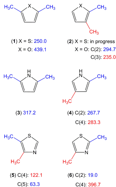
Figure 10. Torsional barriers of the ring methyl rotors in dimethyl-substituted planar five-membered rings (in \text{cm}^{-1} ). (1) X = O: 2,5-dimethylfuran [88], X = S: 2,5-dimethylthiophene [89], (2) X = O: 2,3-dimethylfuran [190], X = S: 2,3-dimethylthiophene, (3) 2,5-dimethylpyrrole [87], (4) 2,4-dimethylpyrrole [191], (5) 4,5-dimethylthiazole [85], and (6) 2,4-dimethylthiazole [192].
