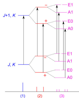
Figure 19. Non-scaled energy levels and microwave signal splittings for molecules featuring one two-fold tunneling motion and a methyl internal rotation, case (3), as in phenyl acetate with rotational
