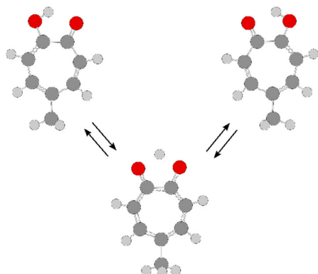
Figure 23. The coupled large amplitude motions of 5-methyltropone. The two equivalent equilibrium conformations shown in the upper trace can be converted into each other over a transition state shown in the lower trace through a hydrogen-transfer tunneling path. This induces a “corrective internal rotation” [215] of 60^\circ for the methyl torsion.
