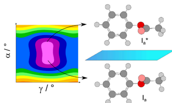
Figure 20. The coupled large amplitude motions of phenyl acetate. Left hand side: 1/6 of the potential energy surface calculated at the MP2/6-311++G(d,p) level of theory demonstrating the methyl and the phenyl torsions ( \alpha and \gamma , respectively). Right hand side: Two equivalent minima of phenyl acetate, reflecting the equilibrium configuration I_a and its mirror image I_a^* . The inversion-tunneling motion connects these two minima.
