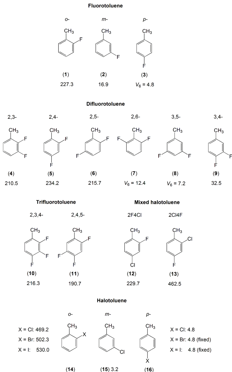
Figure 7. Barriers to methyl internal rotation in halogen-substituted toluene derivatives (in \text{cm}^{-1} ). (1) o-fluorotoluene [161], (2) m-fluorotoluene [162,163], (3) p-fluorotoluene [164], (4) 2,3-difluorotoluene [165], (5) 2,4-difluorotoluene [166], (6) 2,5-difluorotoluene [167], (7) 2,6-difluorotoluene [168], (8) 3,5-difluorotoluene [168], (9) 3,4-difluorotoluene [163,169], (10) 2,3,4-trifluorotoluene [170], (11) 2,4,5-trifluorotoluene [170], (12) 2-fluoro-4-chlorotoluene [129], (13) 2-chloro-4-fluorotoluene [130], (14) o-X-toluene [128], (15) m-chlorotoluene [171], (16) p-X-toluene [172], X = Cl, Br, I.
