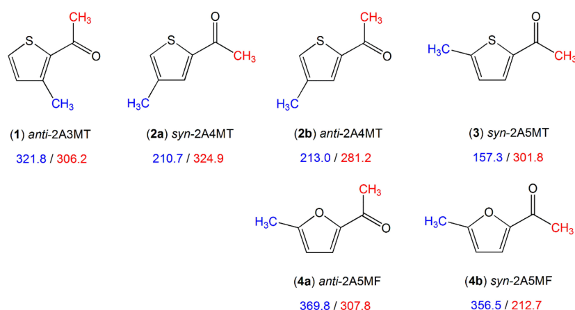
Figure 11. Barriers to methyl internal rotation in furan and thiophene derivatives with a methyl rotor on the ring and an acetyl group which contains another methyl rotor (in \text{cm}^{-1} ). (1) anti -2-acetyl-3-methylthiophene [193], (2) 2-acetyl-4-methylthiophene [194], (3) syn -2-acetyl-5-methylthiophene [195], (4) 2-acetyl-5-methylfuran [86].
