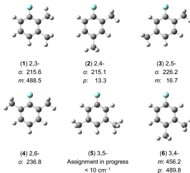
Figure 15. Torsional barriers of the methyl groups in six isomers of dimethylfluorobenzene (in \text{cm}^{-1} ). (1) 2,3-dimethylfluorobenzene [78], (2) 2,4-dimethylfluorobenzene [201], (3) 2,5-dimethylfluorobenzene [202], (4) 2,6-dimethylfluorobenzene [80], (5) 3,5-dimethylfluorobenzene, and (6) 3,4-dimethylfluorobenzene [79].
