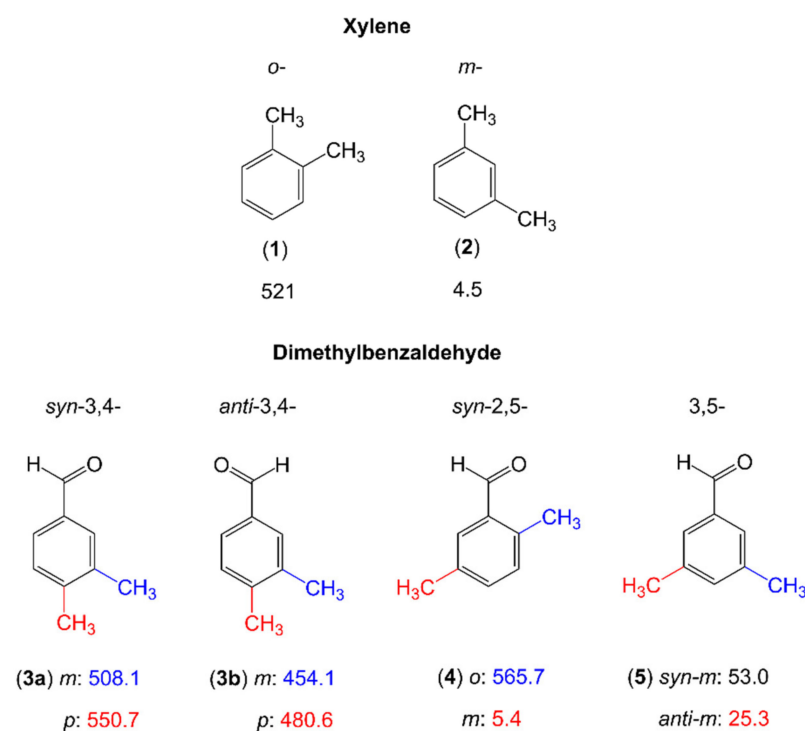
Figure 13. Barriers to methyl internal rotation in xylenes and dimethylbenzaldehydes (in \text{cm}^{-1} ). (1) o -xylene [196], (2) m -xylene [197], (3) 3,4-dimethylbenzaldehyde [81], (4) 2,5-dimethylbenzaldehyde [81], 3,5-dimethylbenzaldehyde [81].
