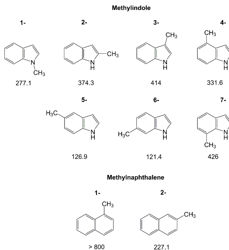
Figure 9. Barriers to methyl internal rotation in large aromatic rings (in \text{cm}^{-1} ). (1) 1-Methylindole [188], (2) 2-methylindole [188], (3) 3-methylindole [188], (4) 4-methylindole [188], (5) 5-methylindole [188], (6) 6-methylindole [188], (7) 7-methylindole [188], (8) 1-methylnaphthalene [131], (9) 2-methylnaphthalene [131].
