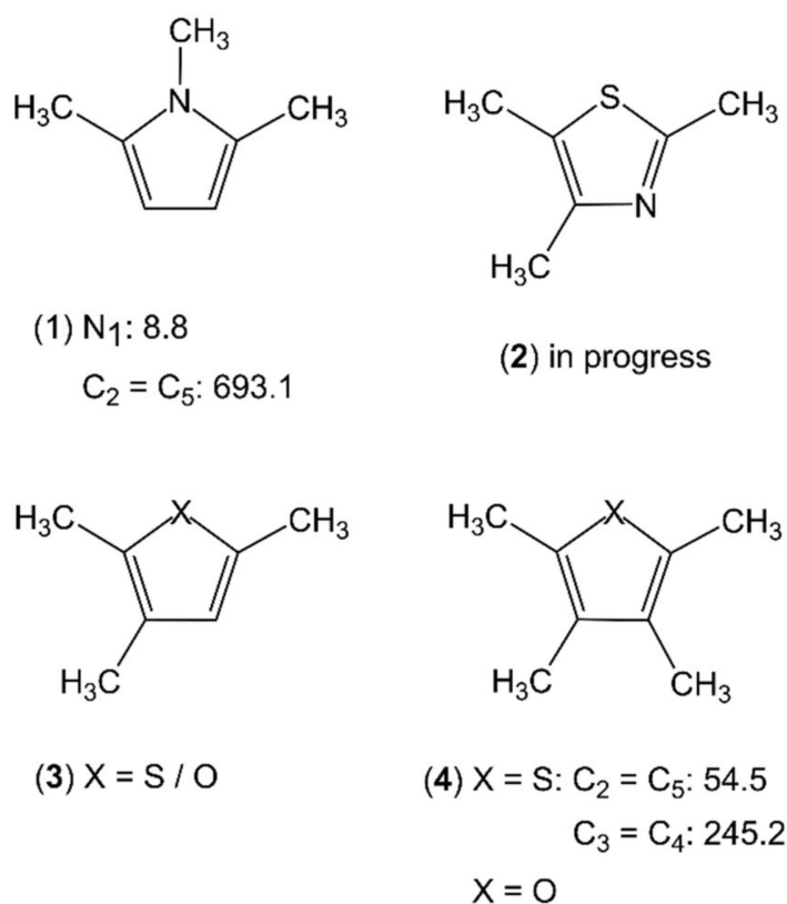
Figure 16. Torsional barriers of the ring methyl rotors in trimethyl- and tetramethyl-substituted planar five-membered rings (in \text{cm}^{-1} ). (1) 1,2,5-trimethylpyrrole [27], (2) 2,4,5-trimethylthiazole, (3) X = O : 2,3,5-trimethylfuran, X = S : 2,3,5-trimethylthiophene, and (4) X = O : 2,3,4,5-tetramethylfuran, X = S : 2,3,4,5-tetramethylthiophene [3,27].
