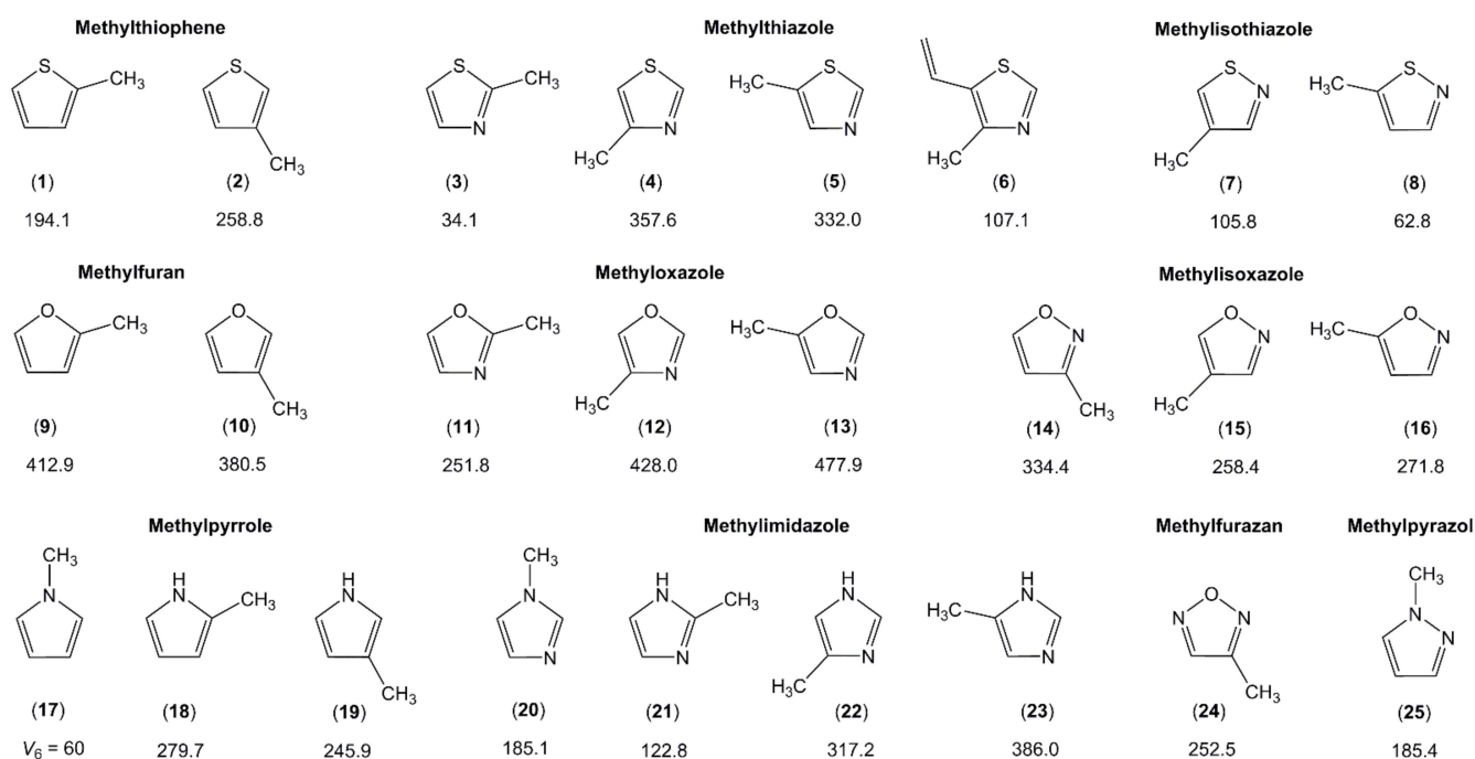
Figure 3. Barriers to methyl internal rotation in monomethyl-substituted planar five-membered rings (in \text{cm}^{-1} ). (1) 2-methylthiophene [96], (2) 3-methylthiophene [97], (3) 2-methylthiazole [98,99], (4) 4-methylthiazole [100], (5) 5-methylthiazole [101], (6) 4-methyl-5-vinylthiazole [102], (7) 4-methylisothiazole [103], (8) 5-methylisothiazole [104], (9) 2-methylfuran [49,105], (10) 3-methylfuran [106], (11) 2-methyloxazole [107], (12) 4-methyloxazole [107,108], (13) 5-methyloxazole [107], (14) 3-methylisoxazole [109], (15) 4-methylisoxazole [110], (16) 5-methylisoxazole [109], (17) N-methylpyrrole [111], (18) 2-methylpyrrole [112], (19) 3-methylpyrrole [113], (20) N-methylimidazole [114], (21) 2-methylimidazole [114], (22) 4-methylimidazole [114], (23) 5-methylimidazole [114], (24) methyl furazan [115], (25) N-methylpyrazole [116].
