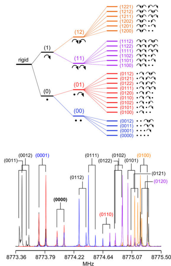
Figure 17. Upper figure: Torsional splittings and spin statistical weights of a rotational transition ( b -type) of 2,3,4,5-tetramethylthiophene. Lower figure: Splittings due to internal rotation of two pairs of equivalent rotors observed in the microwave spectrum of 2,3,4,5-tetramethylthiophene [27].
