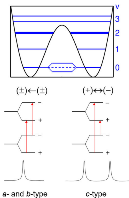
Figure 2. Schematic energy-level diagram illustrating the splittings caused by an inversion-tunneling motion where the \mu_c dipole-moment component changes its sign upon tunneling.
