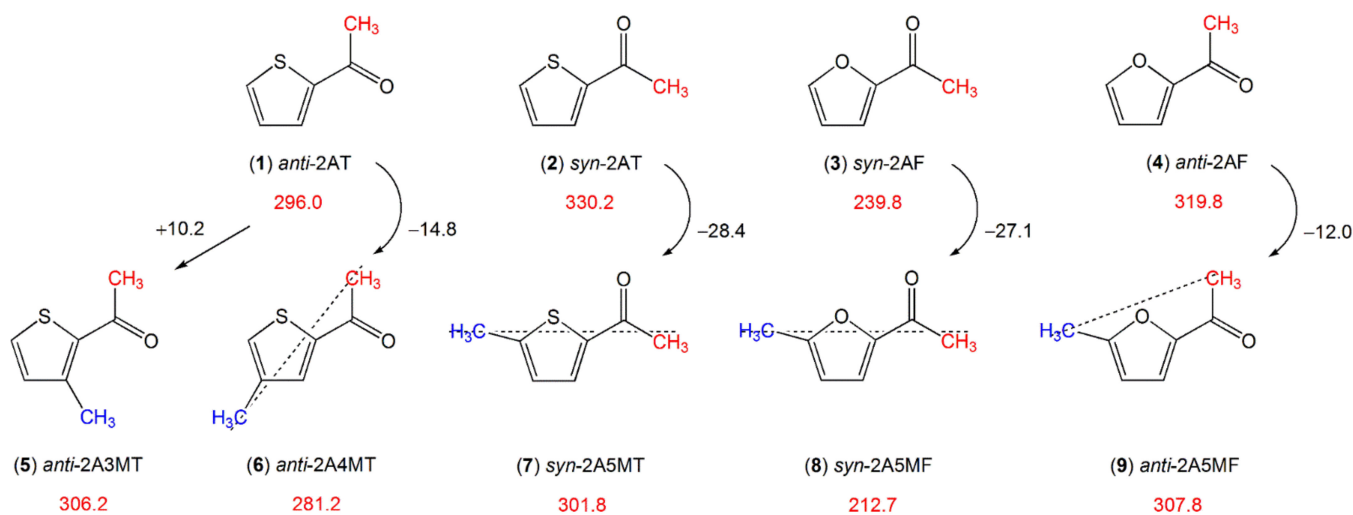
Figure 12. Barriers to methyl internal rotation in furan and thiophene derivatives with an acetyl-group-containing substituent (in \text{cm}^{-1} ). (1) anti -2-acetylthiophene [132], (2) syn -2-acetylthiophene [132], (3) syn -2-acetylfuran [133], (4) anti -2-acetylfuran [133], (5) anti -2-acetyl-3-methylthiophene [193], (6) anti -2-acetyl-4-methylthiophene [194], (7) syn -2-acetyl-5-methylthiophene [195], (8) syn -2-acetyl-5-methylfuran [86], (9) anti -2-acetyl-5-methylfuran [86].
