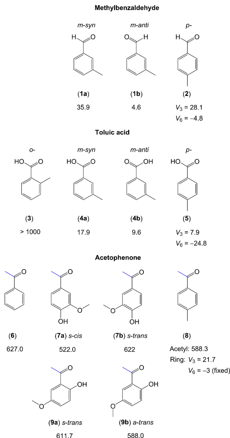
Figure 6. Barriers to methyl internal rotation in toluene derivatives with a carbonyl-containing substituent (in \text{cm}^{-1} ). (1) m-Tolualdehyde [154], (2) p-tolualdehyde [155], (3) o-toluic acid [156], (4) m-toluic acid [157], (5) p-toluic acid [65], (6) acetophenone [158], (7) acetovanillone [159], (8) 4-methylacetophenone [77,160], (9) 6-hydroxy-3-methoxyacetophenone [159].
