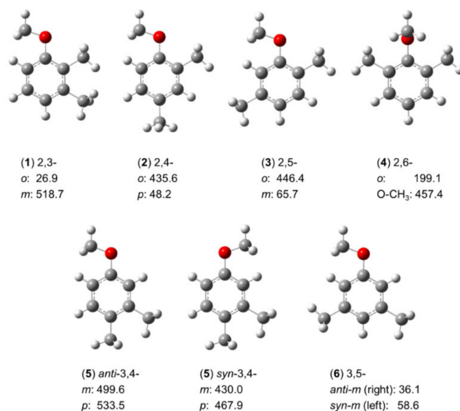
Figure 14. Torsional barriers of the methyl rotors in six isomers of dimethylanisole (in \text{cm}^{-1} ). (1) 2,3-dimethylanisole [84], (2) 2,4-dimethylanisole [82], (3) 2,5-dimethylanisole [198], (4) 2,6-dimethylanisole [198,199], (5) 3,4-dimethylanisole [83], and (6) 3,5-dimethylanisole [198].
