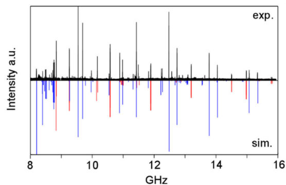
Figure 22. Upper trace: The broadband scan from 8 to 16 GHz of phenyl thioacetate. Lower trace: A predicted spectrum calculated using the parameters of an A0/E0 fit with a standard deviation of 3 MHz. The A species lines are in red, the E species lines in blue [198].
