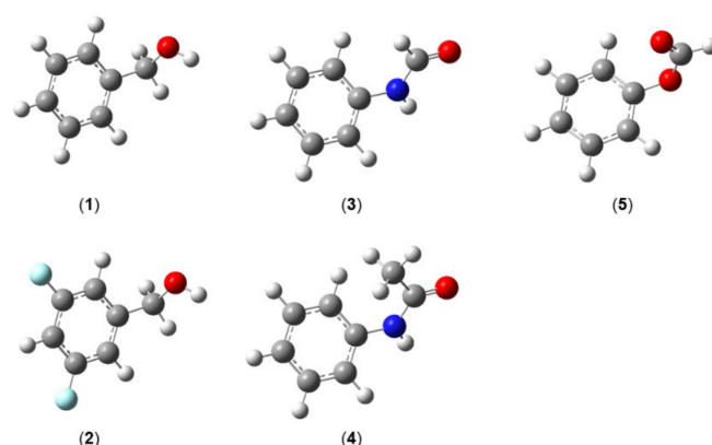
Figure 18. Molecules featuring an inversion-tunneling motion of the phenyl ring. (1) Benzyl alcohol [206], (2) 3,5-difluorobenzyl alcohol [207], (3) E -phenylformamide [208], (4) cis -acetanilide [209], and (5) phenylformate [210].
