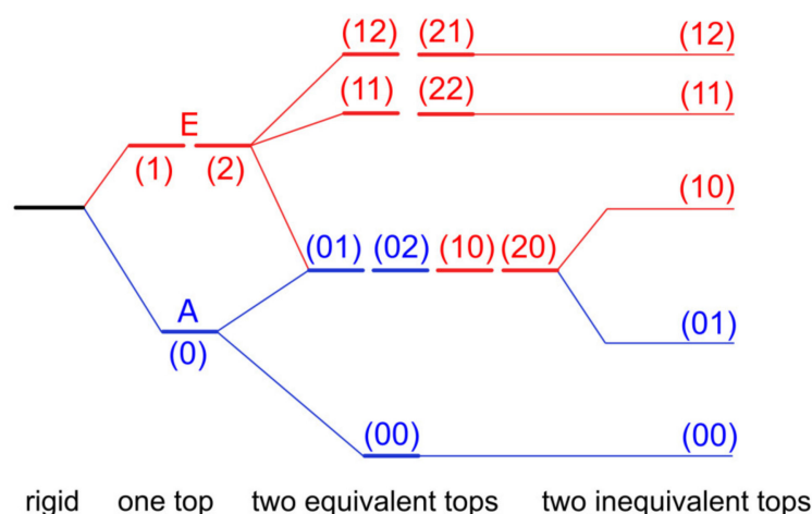
Figure 1. Schematic energy-level diagram illustrating the splittings caused by internal rotation for (i) a rigid rotor (no torsional splitting), (ii) a molecule containing one methyl rotor (splitting into an A and a doubly degenerate E torsional-symmetry species), (iii) a molecule containing two equivalent methyl rotors (splitting into four torsional species), and (iv) a molecule containing two inequivalent methyl rotors (splitting into five torsional species). The three torsional states of the methyl top are given as \sigma = 0, 1, 2 [28]. The (11) and (12) species are not degenerate due to top–top interactions.
