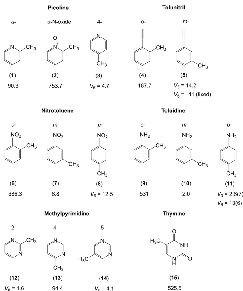
Figure 8. Barriers to methyl internal rotation in nitrogen-containing aromatic six-membered ring (in \text{cm}^{-1} ). (1) \alpha -picoline [173,174], (2) \alpha -picoline-N-oxide [175], (3) 4-picoline [176], (4) o-tolunitril [177,178], (5) m-tolunitril [179], (6) o-nitrotoluene [180], (7) m-nitrotoluene [181], (8) p-nitrotoluene [180], (9) o-toluidine [182], (10) m-toluidine [182], (11) p-toluidine [183], (12) 2-methylpyrimidine [184], (13) 4-methylpyrimidine [185], (14) 5-methylpyrimidine [186], (15) thymine [187].
