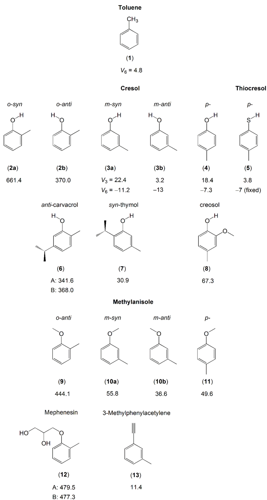
Figure 5. Barriers to methyl internal rotation in toluene and cresol derivatives (in \text{cm}^{-1} ). (1) The prototype toluene [137–142], (2) o-cresol [143], (3) m-cresol [144], (4) p-cresol [145], (5) p-thiocresol [146], (6) anti-carvacrol (two conformers, A and B) [147], (7) syn-thymol [147], (8) creosol [148], (9) o-methyl anisole [127], (10) m-methyl anisole [149,150], (11) p-methylanisole [151], (12) mephesisin (two conformers, A and B) [152], (13) 3-methylphenylacetylene [153].
