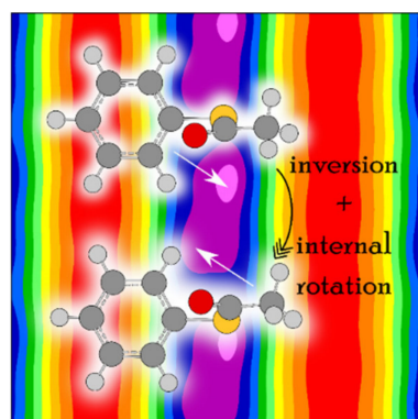
Figure 21. Front layer: View onto the phenyl ring of phenyl thioacetate, showing that: (i) The phenyl ring is almost perpendicular to the C-(C=O)-S plane, and (ii) there are two equivalent structures, corresponding to the inversion tunneling of the phenyl ring (or the thioacetyl group). Back layer: The potential energy surface of phenyl thioacetate calculated at the MP2/6-311++G(d,p) level of theory. The minima are extremely flat and asymmetric [198].
