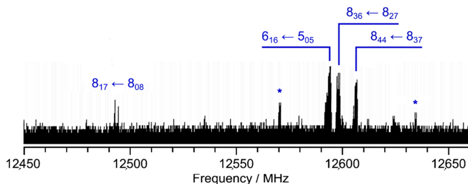
Figure 2. A portion of the survey spectrum of BTA in the frequency range from 12,450 to 12,660 MHz, showing hyperfine splittings arising from the ^{14}\text{N} nuclear quadrupole coupling. Assigned lines are labelled by their rotational quantum numbers J''_{K''_a K''_c} \leftarrow J'_{K'_a K'_c} and all belong to the main isotopologue of BTA. Lines marked with an asterisk are from impurities, as they disappeared when being remeasured later, probably due to a higher vapor pressure than that of BTA.
