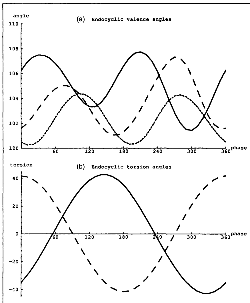
FIGURE 3. Endocyclic valence and torsion angles from CINFLEX at \nu_m = 39^\circ . (a) Valence angles, \theta_1 , O 1 '-C 1 '-C 2 ' (solid line), \theta_2 , C 1 '-C 2 '-C 3 ' (dashed line), and \theta_3 , C 2 '-C 3 '-C 4 ' (dotted line). (b) Torsion angles, \tau_1 , O 1 '-C 1 '-C 2 '-C 3 ' (solid line), and \tau_2 , C 1 '-C 2 '-C 3 '-C 4 ' (dashed line).
