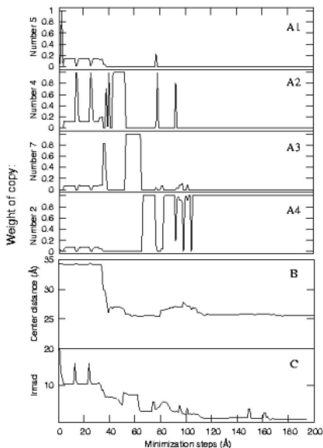
Fig. 2. Variations of the copy weight (A 1–4), the distance between geometric centers of the receptor and the ligand (B) and the Lrmsd value (RMSD of the ligand with respect to its position in the crystal complex) (C) versus minimization step during a typical docking minimization (for one starting configuration). The copy ensemble is composed of ten loop copies, but for clarity only four copies are represented in the graphs A1, A2, A3, and A4 (the six others copies present low weight during the major part of the minimization). During the 73 first steps of minimization, a force constant is applied between the two partners in order to generate a tight complex. At the beginning of the simulation, copy weights are almost equivalent because the ligand is far away from the receptor. However, the ligand approach favors the copy number 7. When the ligand adjusts to the receptor, the copy number 2 is finally selected (weight equal to 1).
