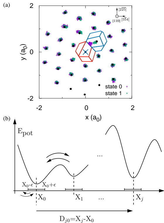
Figure 1. (Color online) (a) A collection of 84 microstates projected on the plane perpendicular to the tilt axis of the \Sigma 33(554)[110] symmetrical tilt boundary, in Al, under 3% strain. Only the positions (small crosses) in the vicinity of the vacancy (large cross) and within two (220) layers containing the vacancy are shown. The black dots are the lattice sites (the edges of two Voronoi cells [41] are also shown). (b) Schematic illustration of the Smart Darting method. X_j is a local minimum of the potential energy, \epsilon is the radius of the spheres around the minima.
