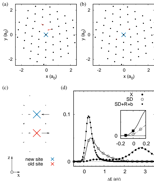
Figure 3. (Color online) Relaxations around a single vacancy (large cross) on the most favorable site of the \Sigma 33(554)[110] symmetrical tilt grain boundary, strained by 3% perpendicular to its plane. (a) State 0 (“delocalized vacancy”) and (b) state 1 (“localized vacancy”). Displacement values larger than 0.05 a_0 are represented by arrows. They constitute, together with the site index, the topology used for the Smart Darting moves. (c) Vectors represent the “dart” for moving the vacancy along the tilt axis by one period. (d) Distribution of the energy variation \Delta E (eV) when a simple exchange (X), a simple Smart Darting exchange (SD) or a Smart Darting exchange plus the sampling of the neighbors, including the bias in the acceptance rule -kT \log \frac{\prod (n \rightarrow o)}{\prod (o \rightarrow n)} (SD+R+b) (Eq. 7), are made. Only neighbors with a relaxation larger than 0.1 a_0 were considered and the acceptance rate was on the order of 5% at T=300 K.
