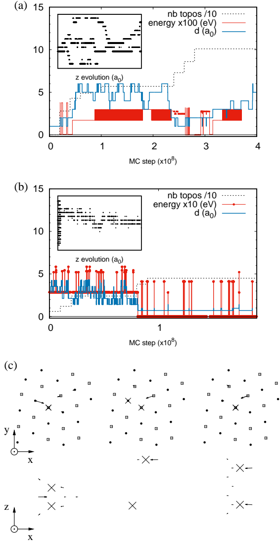
Figure 6. (Color online) Evolution of the distance between the vacancies, the energy of the topology visited and the number of topologies detected along the Markov chain for a system containing two vacancies: (a) \Sigma 13(320)[001] at T=300 K, (b) \Sigma 33(554)[110] at T=600 K both in Al. The position in z (the tilt axis direction) is shown on the insert. (c) The three main topologies visited in (b) with energies 0 eV, 0.52 eV and 0.28 eV from left to right.
