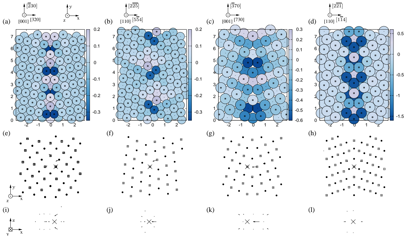
Figure 5. (Color online) Symmetrical tilt grain boundary structures without vacancies: (a) \Sigma 13(320)[001] , (b) \Sigma 33(5\bar{5}4)[110] in Al and (c) \Sigma 29(730)[001] , (d) \Sigma 9(1\bar{1}4)[110] in bcc Fe. Colors represent the vacancy segregation energy ( \Delta E_{seg} ). The minimum values are given in table II. The relaxations around a single vacancy in this optimal configuration are represented by arrows on (e,f,g,h) projected in the (x,y) plane and in the (x,z) plane on (i,j,k,l) (only the displacements are shown). The vacant site is marked by a large cross.
