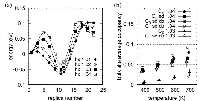
Figure 4. (a) Energy profile between state 1 (replica 0) and state 0 (replica 11) obtained by the NEB, as a function of the homothety factor applied perpendicular to the GB. (b) Occupancy of a bulk site when it is put in equilibrium with the GB either in state 0 or in state 1, as a function of temperature and for two strain levels hx=1.03 and hx=1.04 .
