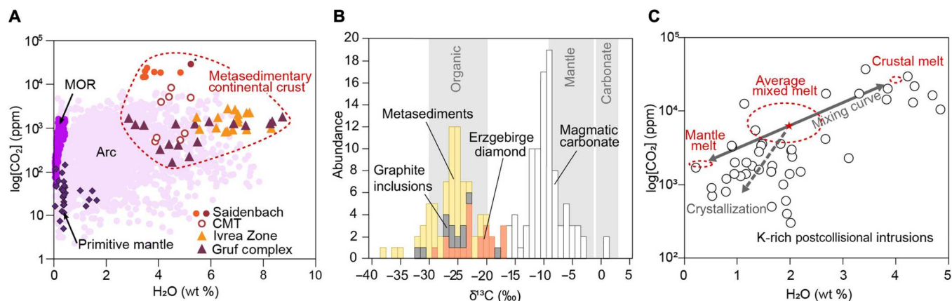
Fig. 4. Volatiles content in melt inclusions. (A) \text{H}_2\text{O} (wt %) and \text{CO}_2 (ppm) content of glass and a rehomogenized (indicated with an asterisk) nanogranitoid from Saldenbach eclogites measured and corrected by NanoSIMS (error bar smaller than the symbol) and compared with \text{H}_2\text{O} and \text{CO}_2 contents of lower continental crust melt inclusions in granulites [Central Maine Terrane (CMT) (19), Ivrea Zone (20), and Gruf Complex (61)]. See table S5 for volatiles data, and for NanoSIMS calibration curves, see fig. S1. Primitive mantle, mid-oceanic ridges (MOR), and arc volcanoes after (13). The dashed area indicates the compositions of melt derived from the metasedimentary continental crust. (B) Carbon isotopic compositions in the Erzgebirge [see table S6 for \delta^{13}\text{C} data of carbonate (76), calcite (75, 77, 95), and dolomite (77) of postcollisional mineralization and of diamond in garnet (66), whole rock (68), and graphite in zircon (65) of metasediments of the Erzgebirge]. Shaded areas for the range of organic and carbonate \delta^{13}\text{C} values after (70). The mantle values are from (71). (C) \text{CO}_2 and \text{H}_2\text{O} content of mantle and crustal melt mixing compared with potassium-rich postcollisional intrusions in the Bohemian Massif (empty circles) (96–99). See table S7 for \text{CO}_2 and \text{H}_2\text{O} data of (ultra)potassic magmatic rocks. The star indicates the average composition of the calculated melt. The dashed arrow indicates the inferred general decrease in melt \text{CO}_2 and \text{H}_2\text{O} concentration during ascent and cooling due to the increase in melt/fluid immiscibility and the partition of volatile species between these two phases.
