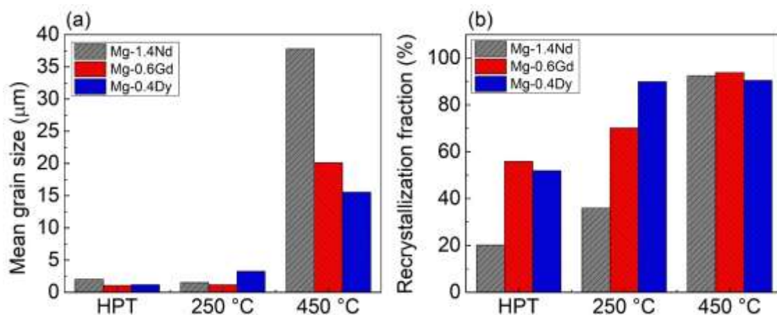
Figure 3: Evolution of: (a) mean grain size and (b) recrystallization fraction of HPT-processed and annealed Mg-1.4Nd, Mg-0.6Gd and Mg-0.4Dy alloys at 250 and 450 °C for 1 h, respectively.
