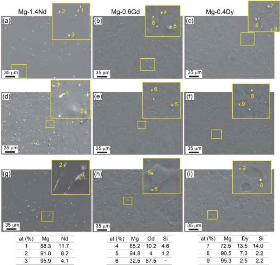
Figure 5: SEM photos of HPT-processed (a) Mg-1.4Nd, (b) Mg-0.6Gd, (c) Mg-0.4Dy, annealed at 250 °C for 1 h: (d) Mg-1.4Nd, (e) Mg-0.6Gd, (f) Mg-0.4Dy and annealed at 450 °C for 1 h: (g) Mg-1.4Nd, (h) Mg-0.6Gd, and (i) Mg-0.4Dy alloys.
