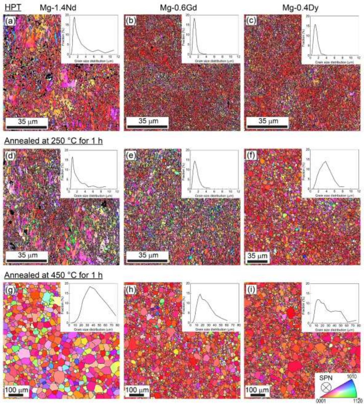
Figure 2: SPN-IPF maps and grain size distributions of HPT-processed : (a) Mg-1.4Nd, (b) Mg-0.6Gd, (c) Mg-0.4Dy, annealed at 250 °C for 1 h: (d) Mg-1.4Nd, (e) Mg-0.6Gd, (f) Mg-0.4Dy and annealed at 450 °C for 1 h: (g) Mg-1.4Nd, (h) Mg-0.6Gd, and (i) Mg-0.4Dy alloys. The HAGBs are indicated by a black line. SPN denotes the shear plane normal direction.
