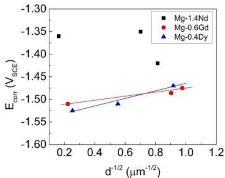
Figure 10: Evolution of E_{corr} as a function of d^{-1/2} for HPT-processed and annealed Mg-1.4Nd, Mg-0.6Gd and Mg-0.4Dy samples.
