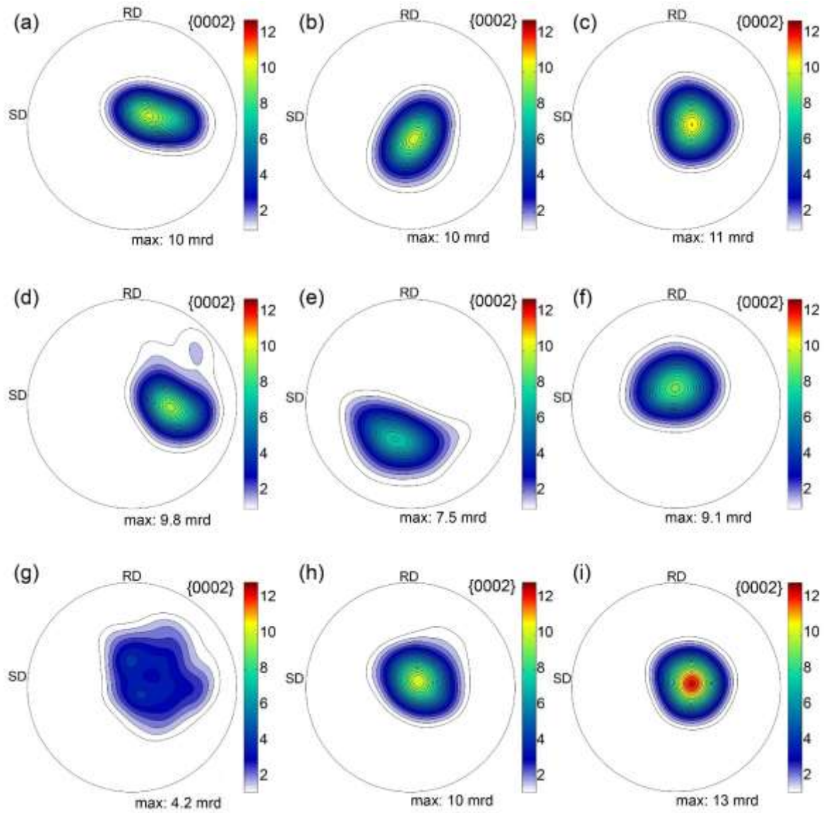
Figure 6: Evolution of texture presented by the recalculated \{0002\} pole figures of the HPT-processed : (a) Mg-1.4Nd, (b) Mg-0.6Gd, (c) Mg-0.4Dy, annealed at 250 °C for 1 h: (d) Mg-1.4Nd, (e) Mg-0.6Gd, (f) Mg-0.4Dy and annealed at 450 °C for 1 h: (g) Mg-1.4Nd, (h) Mg-0.6Gd, and (i) Mg-0.4Dy alloys.
