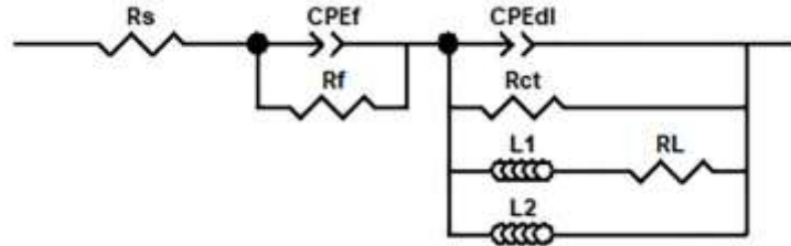
Figure 8: Equivalent electric circuit used to fit the Nyquist plots of HPT-processed and annealed Mg-RE samples.
