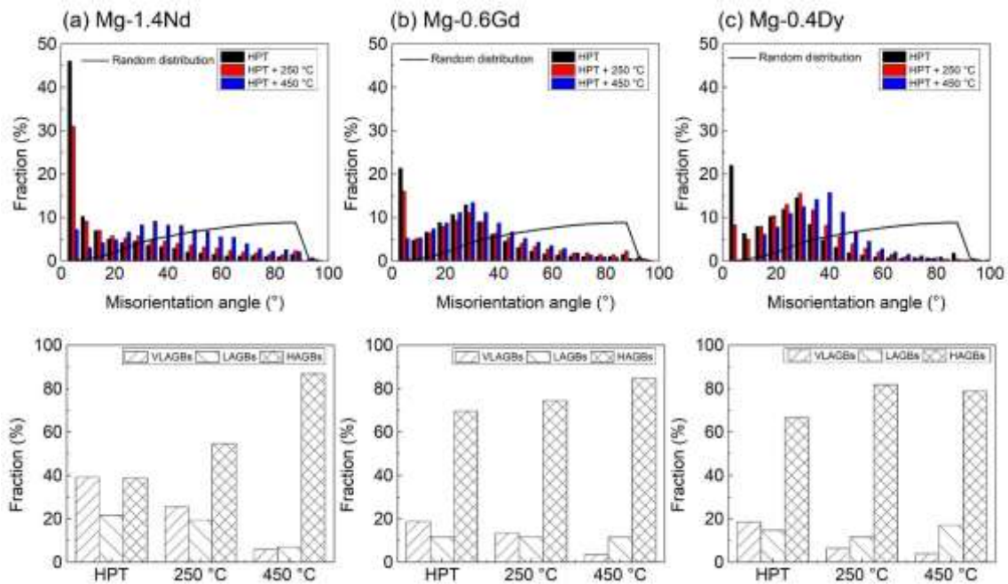
Figure 4: Grain boundary misorientation angle distributions and fractions of VLAGBs, LAGBs, and HAGBs of samples HPT-processed and annealed at 250 and 450 °C for 1 h: (a) Mg-1.4Nd, (b) Mg-0.6Gd and (c) Mg-0.4Dy alloys.
