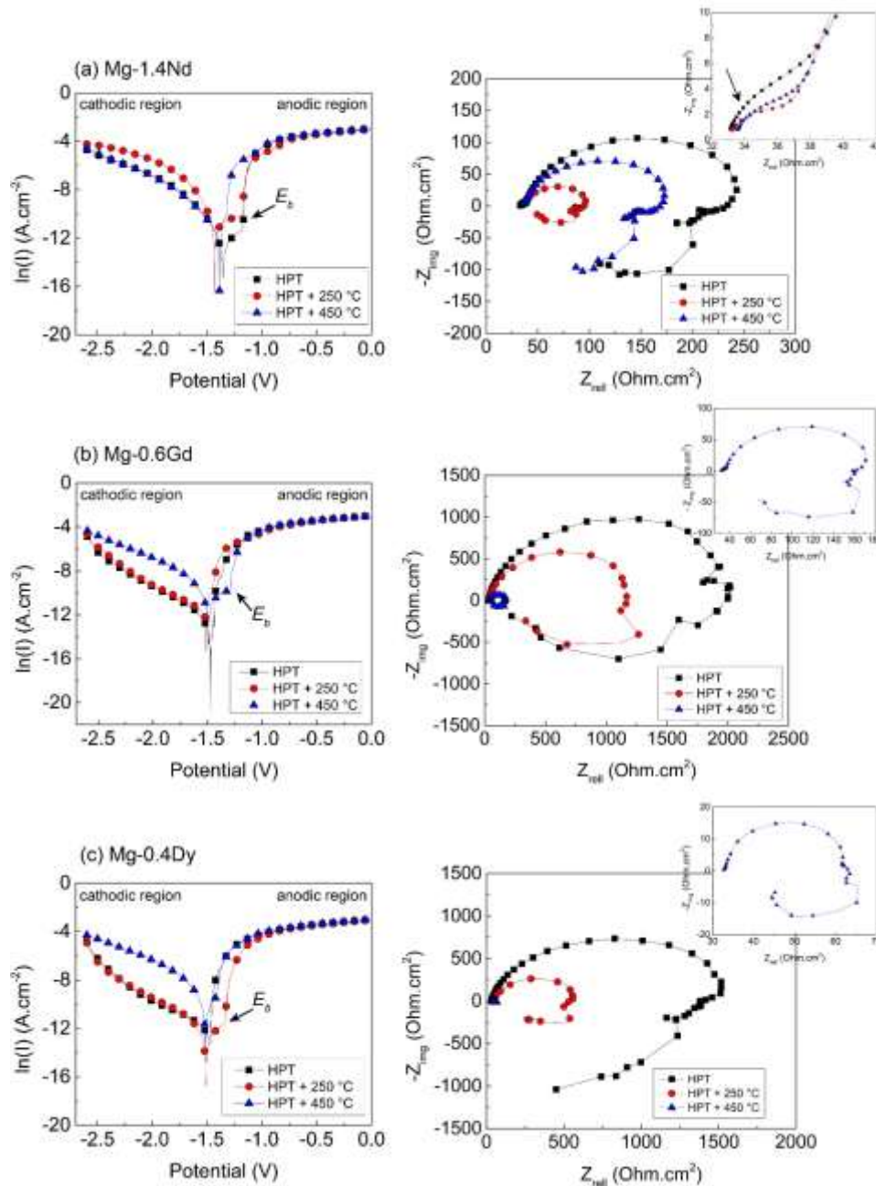
Figure 7: Polarization curves and Nyquist plots in a 3.5 % NaCl solution of deformed and recrystallized samples of: (a) Mg-1.4Nd, (b) Mg-0.6Gd and (c) Mg-0.4Dy alloys. The Nyquist plots of the HPT-processed and annealed Mg-1.4Nd (250 and 450 °C), annealed Mg-0.6Gd at 450 °C and Mg-0.4Dy at 450 °C are placed at the upper right with a small scale for further visibility.
