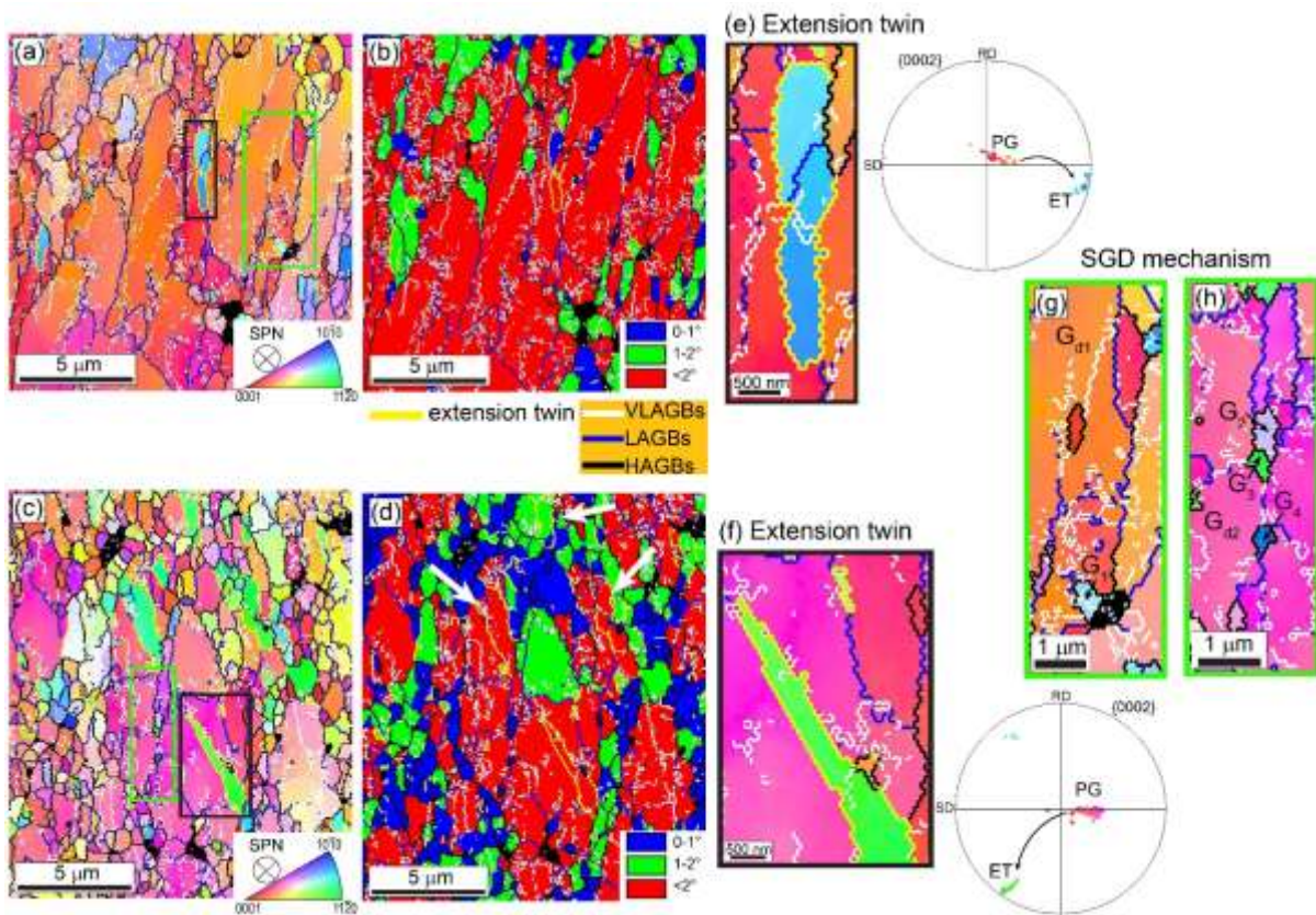
Figure 9: IPF and GOS maps of selected regions from the microstructures of: (a, b) HPT-processed (from Figure 2) and (c, d) annealed Mg-1.4Nd at 250 °C for 1 h (from Figure 2) showing the presence of (e and f) an extension twin (black box) and corresponding {0002} pole figure and (g, h) a sub-grain development mechanism (green box).
