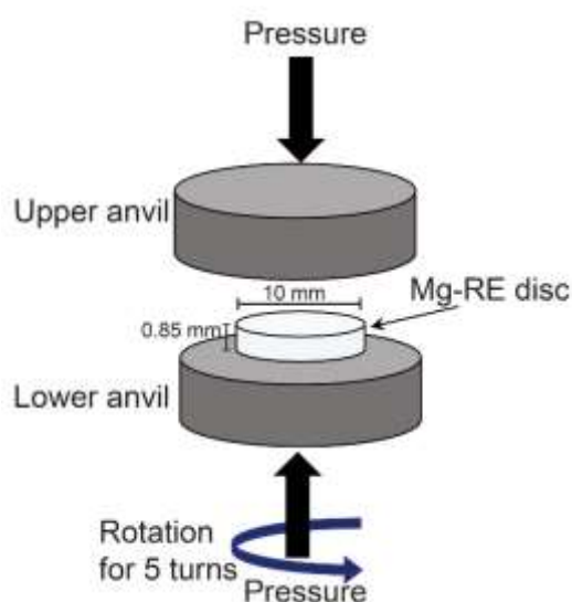
Figure 1: Schematic illustration showing the HPT processing.
