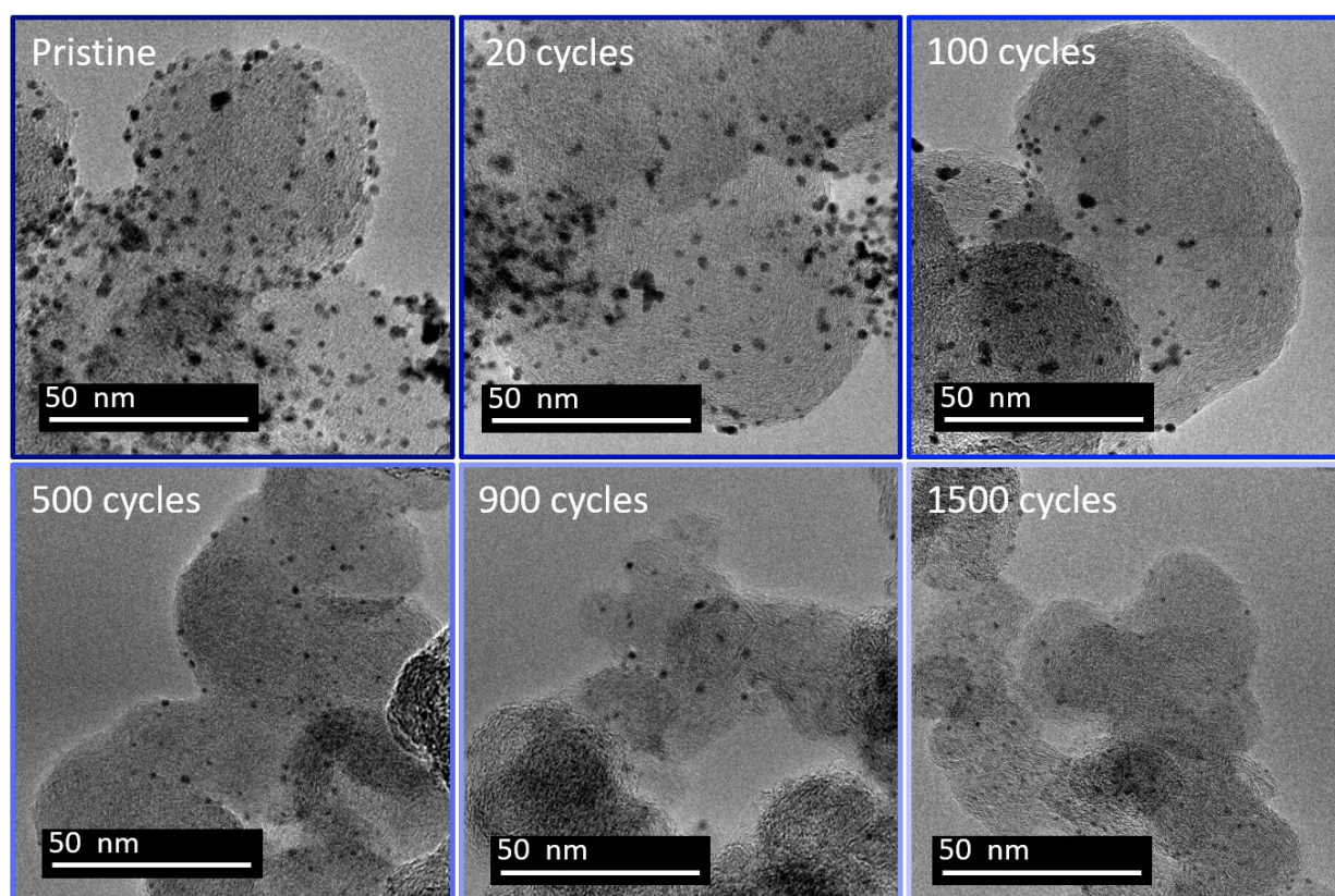
Fig. 3 Representative TEM images of platinum particles from a Pt/C 20% TTK at 20 \mu\text{g cm}^{-2} loading at different stage of cycling between 1.2 and 0.85 V vs RHE in 1 M \text{H}_2\text{SO}_4 + 0.01 M NaCl.
