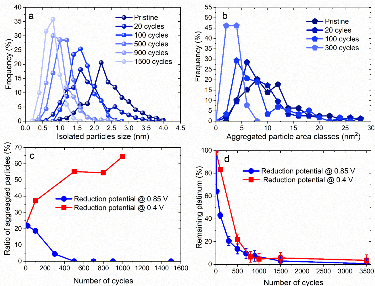
Fig. 4 Distribution of particle size and area for a) isolated particles and b) aggregated particles. These parameters are evaluated at different stage of the cycling protocol between 0.85 and 1.2 V vs RHE in 1 M H 2 SO 4 + 0.01 M NaCl; Comparison between the two reduction potentials 0.4 and 0.85 V vs RHE for c) ratio of the number aggregated particles to the total number of particles and d) the evolution of platinum content remaining on the electrode
