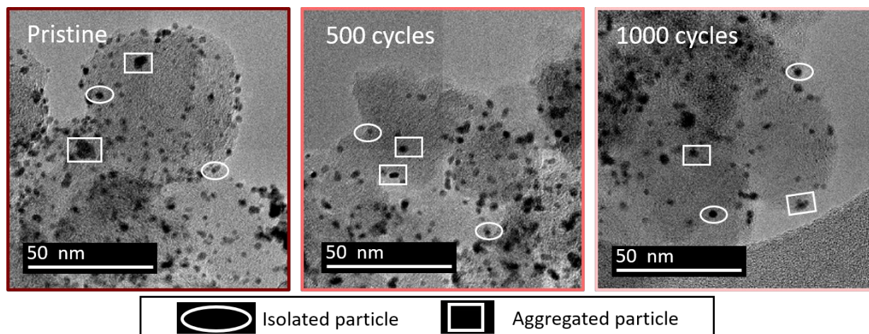
Fig. 1 Representative TEM images of platinum nanoparticles from a Pt/C 20% TKK at 20 \mu\text{g cm}^{-2} loading at different stages of cycling between 1.2 and 0.4 V vs RHE in 1 M \text{H}_2\text{SO}_4 + 0.01 M NaCl. The ellipses highlight some examples of isolated particles and the rectangles show some examples of aggregated particles.
