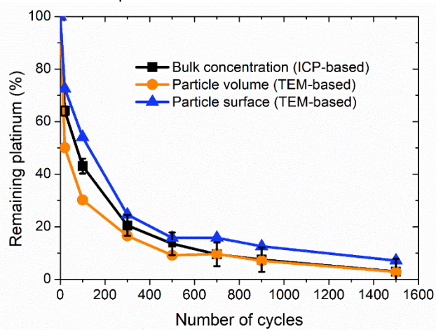
Fig. 5 Comparison of evolution of remaining platinum rate on the electrode as a function of the number of cycles estimated
