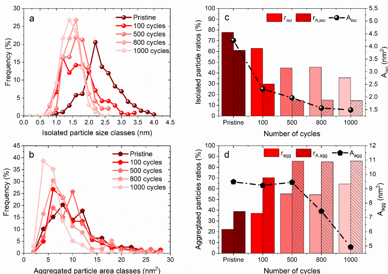
Fig. 2 Distribution of particle a) diameter for isolated particles and b) area for aggregated particles; Parameters and average area for c) isolated particles r_{n,iso} and r_{A,iso} and d) aggregated particles r_{n,agg} and r_{A,agg} are measured from pristine to 1000 cycles. These parameters are evaluated at different stage of the cycling protocol between 0.4 and 1.2 V vs RHE in 1 M H 2 SO 4 + 0.01 M NaCl.
