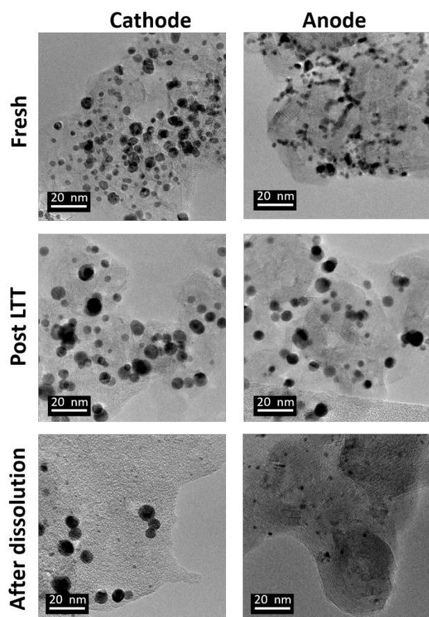
Fig. 6 Representative TEM images of platinum particles for fresh MEA, post LTT MEA and for MEA after Pt electrochemical dissolution protocol consisting in 4000 cycles between 1.2 – 0.85 V vs RHE in 1 M H 2 SO 4 + 0.01 M NaCl.
