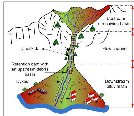
Figure 1: Torrential watershed and structural protection measures.
