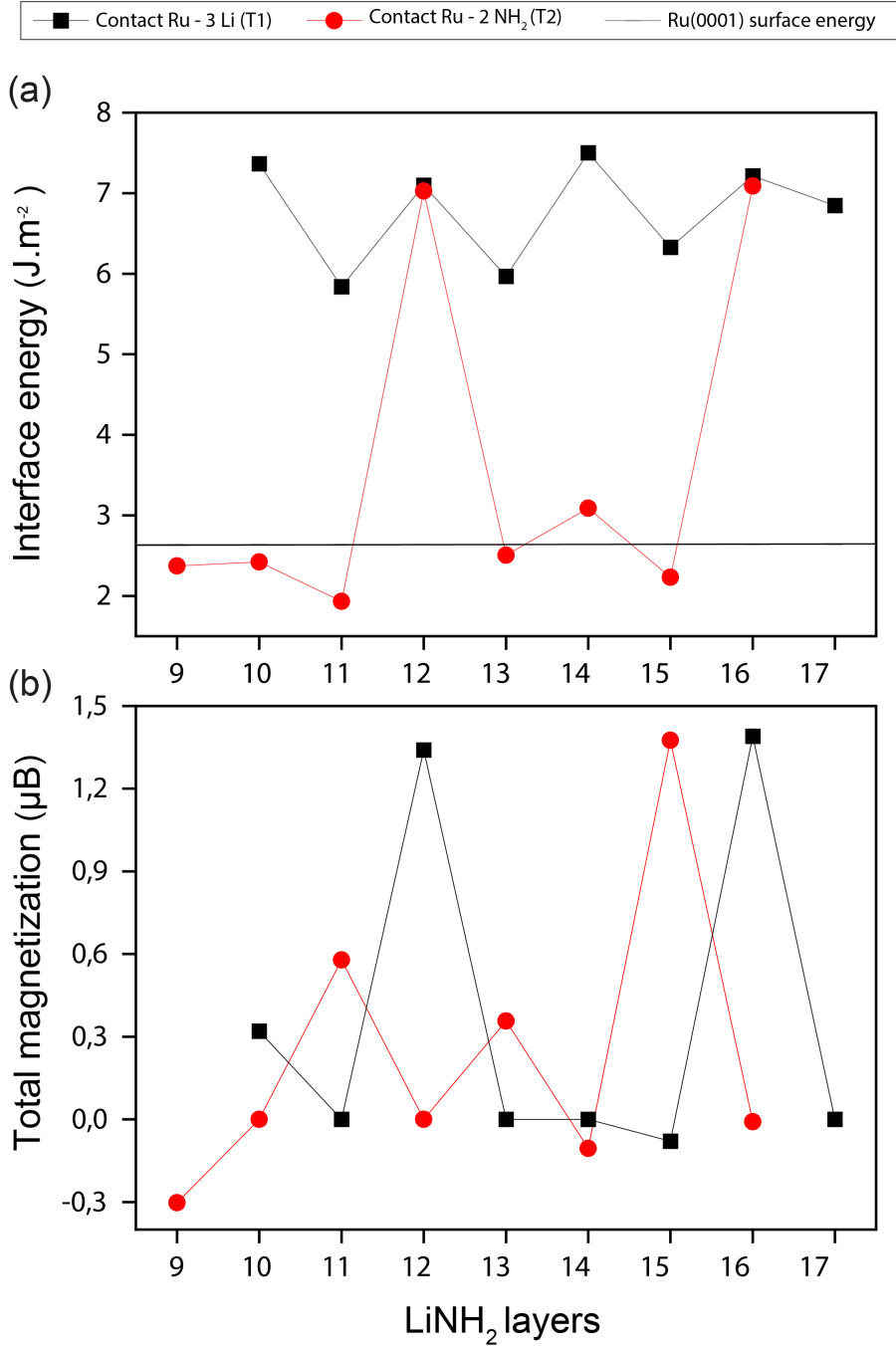
Figure 5: (a) Interface energies ( \text{J}\cdot\text{m}^{-2} ) of optimized Ru(0001)/LiNH 2 (001) systems (GGA PBE) as a function of the thickness of LiNH 2 (001) slab (see Table 4 for details). The two considered contacts between materials is marked by different colors: black for a contact with an atomic Li plane P1 (related to T1 termination) and red for a contact with a NH 2 molecular plane P2 (related to T2 termination). See Figure 1 for definitions of planes in LiNH 2 . For a given thickness, only the interface energy of the most stable model is reported from Table 4. The horizontal black line corresponds to the calculated value of the surface energy of the clean reference Ru(0001). (b) Total magnetization ( \mu\text{B} ) of optimized Ru(0001)/LiNH 2 (001) interfaces (GGA PBE) as a function of the thickness of LiNH 2 (001) slab.
