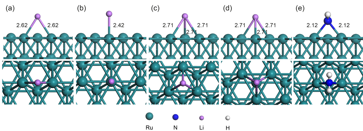
Figure 3: Lateral and top views of optimized adsorption structures of a Li atom on Ru(0001): (a) bridge, (b) top, (c) hollow free and (d) hollow hcp positions. (e) Lateral and top views of the optimal adsorption structure of a bridge-bonded NH 2 fragment on Ru(0001). Distances are addressed in Å. Labels and colors of atoms are depicted.
