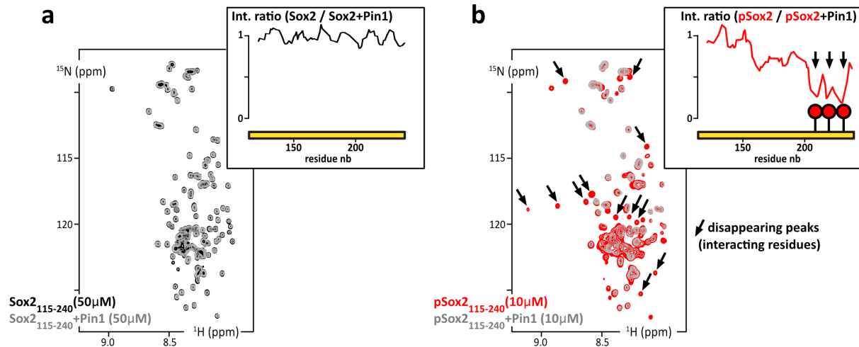
1 2 Figure 7: a. Overlay of 2D ^1\text{H} - ^{15}\text{N} HSQC spectra of ^{15}\text{N} -Sox2(aa115-240) alone at 50 \mu\text{M} (black) or 3 mixed with Pin1 in isotopic natural abundance and in stoichiometric amounts (grey) ; inset up-right : 4 residue specific NMR signal intensity ratios as measured in the two HSQC spectra. b. Overlay of 2D ^1\text{H} - 5 ^{15}\text{N} HSQC spectra of ^{15}\text{N} -phosphoSox2(aa115-240) alone at 10 \mu\text{M} (red) or mixed with the Pin1-WW 6 domain in stoichiometric amounts (grey); insets, up-right : residue specific NMR signal intensity ratios 7 as measured in the two HSQC spectra (in absence/presence of Pin1-WW domain). 8
