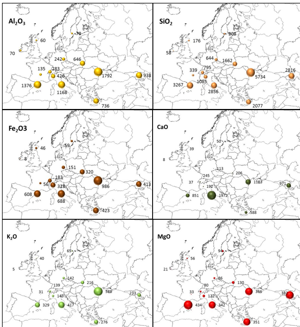
Figure 6.4: Spatial distribution of the mean concentrations of Al_2O_3 , SiO_2 , Fe_2O_3 , CaO , K_2O and MgO (in ng/m^3 ) determined for each site during the June/July 2012 EMEP IMP.
