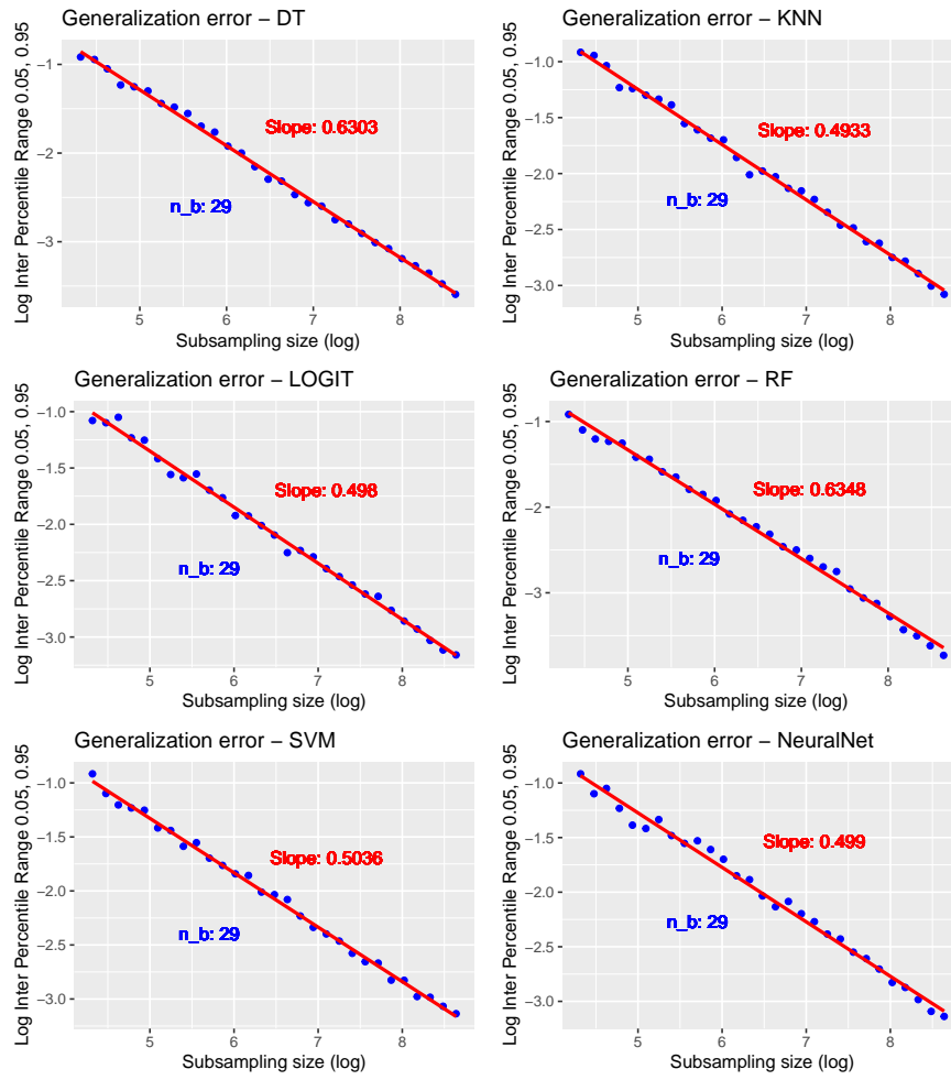
Figure B3. Estimation of convergence rate on IPR90, VeReMi dataset, N = 424,810
