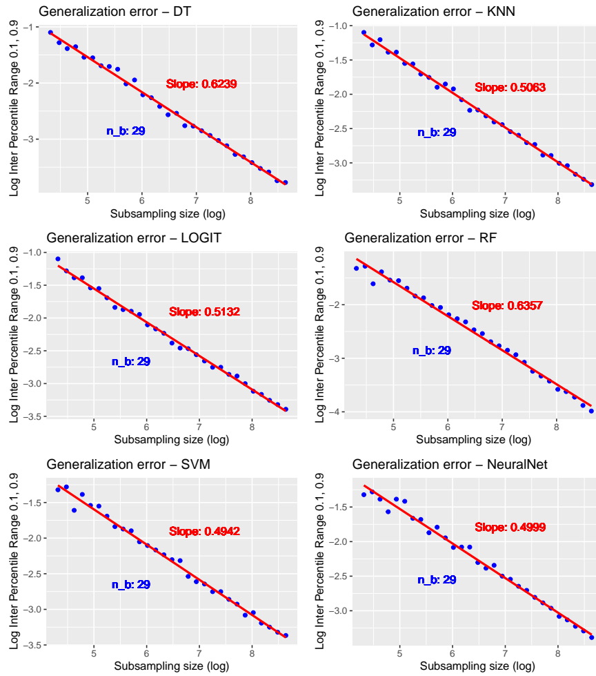
Figure B2. Estimation of convergence rate, based on IPR80, VeReMi dataset, N = 424,810
