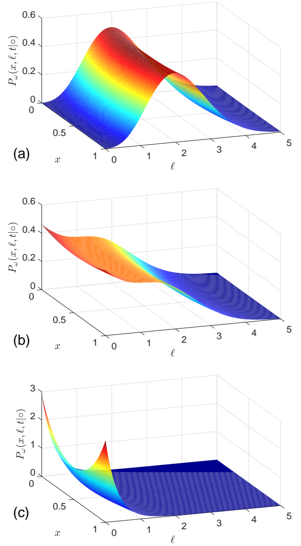
FIG. 6: The regular part of the volume-averaged full propagator P_\omega(x, \ell, t|0) under Poissonian resetting of the boundary local time at rate \omega for diffusion on the unit interval ( b = 1 ), with D = 1 , b = 1 , t = 1 , \omega = 0 (a), \omega = 1 (b), and \omega = 10 (c). P_\omega(x, \ell, t|0) was obtained from Eq. (54) by numerical inversion of the Laplace transform.
