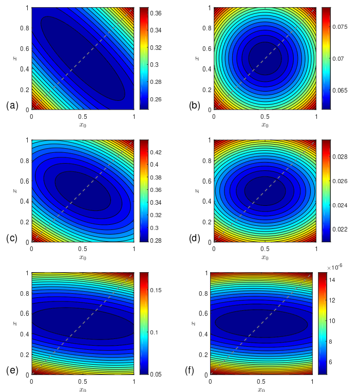
FIG. 8: Colored contour plots of the Laplace-transformed full propagator \tilde{P}_\omega(x, \ell, p|x_0) under Poissonian resetting of the boundary local time at rate \omega for diffusion on the unit interval ( b = 1 ), with D = 1 , p = 1 , \ell = 1 (left column) and \ell = 4 (right column). Panels correspond to \omega = 0 (a,b), \omega = 1 (c,d), and \omega = 10 (e,f).
