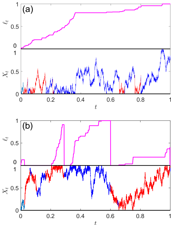
FIG. 1: Simulation of a random trajectory X_t on the unit interval (0,1) and its boundary local time \ell_t under Poissonian resetting with the law \mathbb{P}\{\delta > t\} = \Phi(t) = e^{-\omega t} for the resetting time \delta , with the rate \omega = 10 , the diffusion coefficient D = 1 , and the starting point x_0 = 0 . The boundary local time is rescaled by its maximum and shifted upwards for an easier visualization. (a) Position resetting; (b) Boundary local time resetting. The trajectory is shown by pieces that change color (blue and red) at each resetting.
