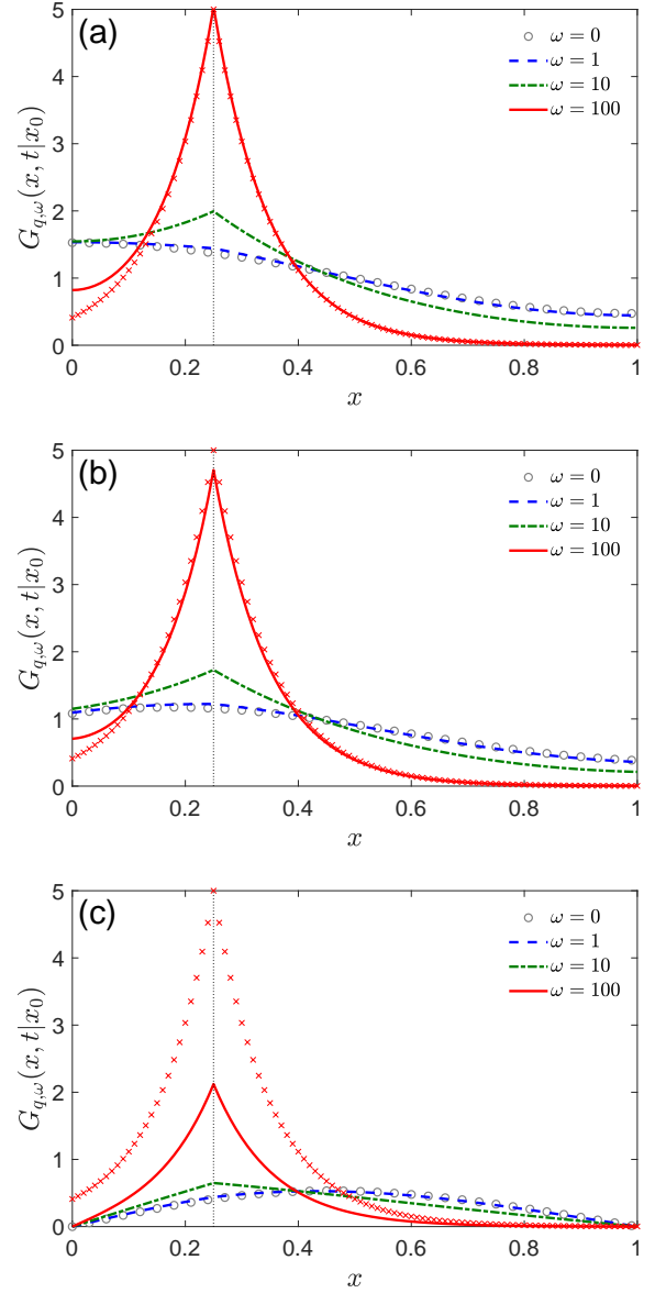
FIG. 2: The propagator G_{q,\omega}(x, t|x_0) under Poissonian resetting of the position at the rate \omega for diffusion on the unit interval ( b = 1 ), with x_0 = 0.25 , t = 0.1 , D = 1 , four values of \omega (see legend), and q = 0 (a), q = 1 (b), and q = \infty (c). Note that \omega = 0 corresponds to the propagator G_q(x, t|x_0) without resetting. Vertical dotted line indicates the position x_0 . Crosses present the steady-state density in Eq. (82) at \omega = 100 for the whole line without any target.
