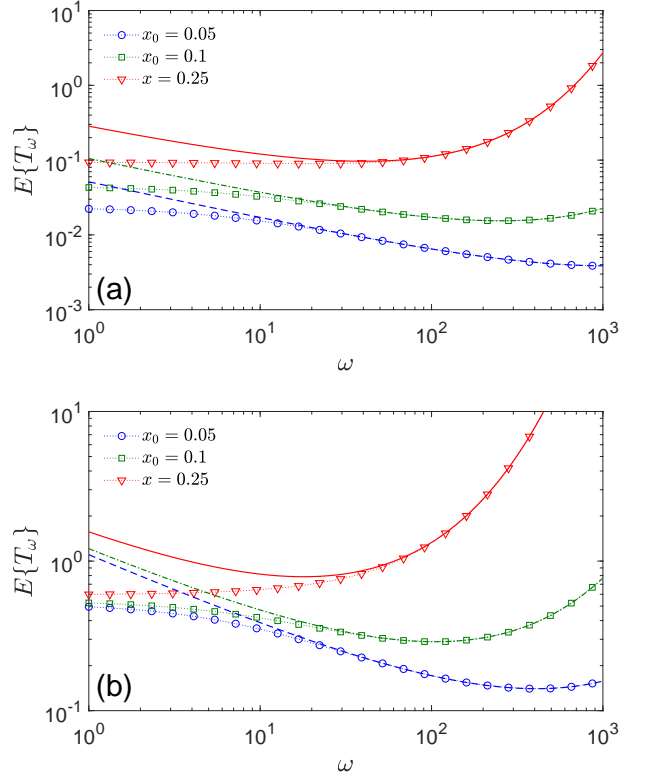
FIG. 3: The mean first-reaction time \mathbb{E}\{\mathcal{T}_{\omega}\} under Poissonian resetting of the position at rate \omega for diffusion on the unit interval ( b = 1 ), with D = 1 , three values of x_0 (see the legend), q = \infty (a) and q = 1 (b). Symbols show the exact result (37) with \tilde{S}_q(p|x_0) from Eq. (73), while lines illustrate the approximate relation (85).
