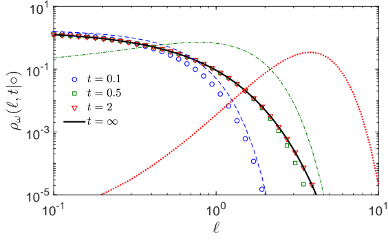
FIG. 5: The regular part of the probability density \rho_\omega(\ell, t|0) of the boundary local time \ell_t under Poissonian resetting, with D = 1 , b = 1 , and several times t (see the legend). Thin lines show the case without resetting ( \omega = 0 ), while symbols present the case with moderate resetting ( \omega = 10 ). A thick black line indicates the steady-state probability density \rho_\omega^{\text{st}}(\ell) from Eq. (61).
