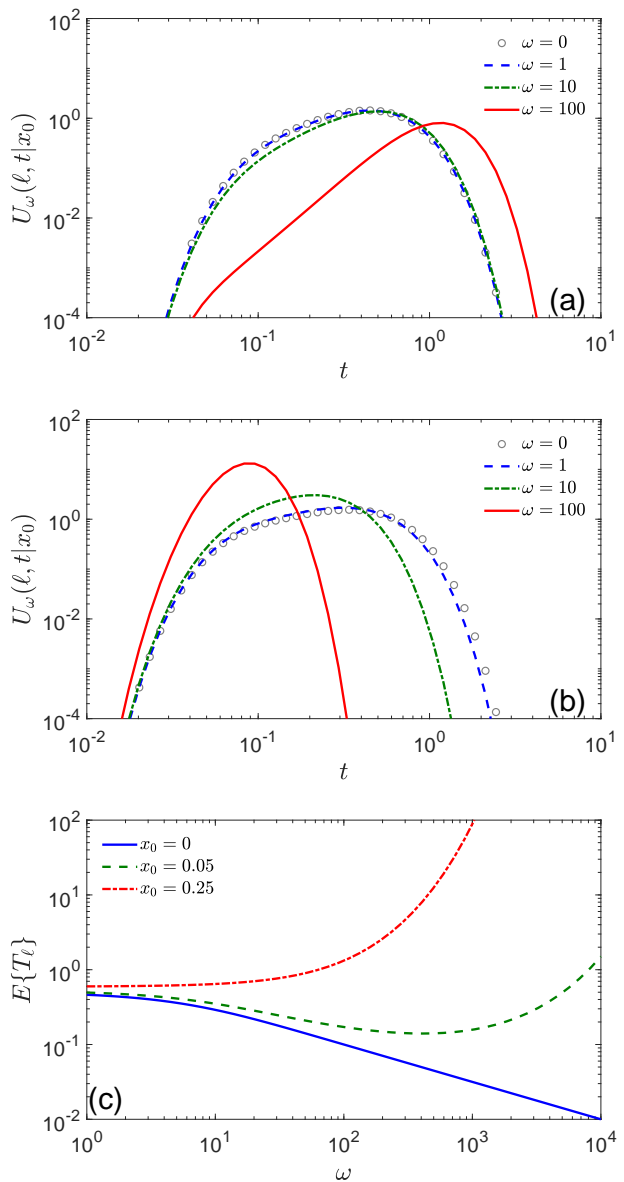
FIG. 4: (a,b) The probability density U_\omega(\ell, t|x_0) of the first-crossing time \mathcal{T}_\ell under Poissonian resetting of the position at the rate \omega for diffusion on the unit interval ( b = 1 ), with D = 1 , \ell = 1 , four values of \omega (see the legend), x_0 = 0.25 (a) and x_0 = 0 (b). The density was obtained by the numerical inversion of the Laplace transform in Eq. (A6) via the Talbot algorithm. (c) The mean first-crossing time \mathbb{E}\{\mathcal{T}_\ell\} under Poissonian resetting as a function of the rate \omega , for \ell = 1 and three values of x_0 (see the legend). \mathbb{E}\{\mathcal{T}_\ell\} was obtained as the derivative of Eq. (A6) with respect to p , evaluated at p = 0 .
