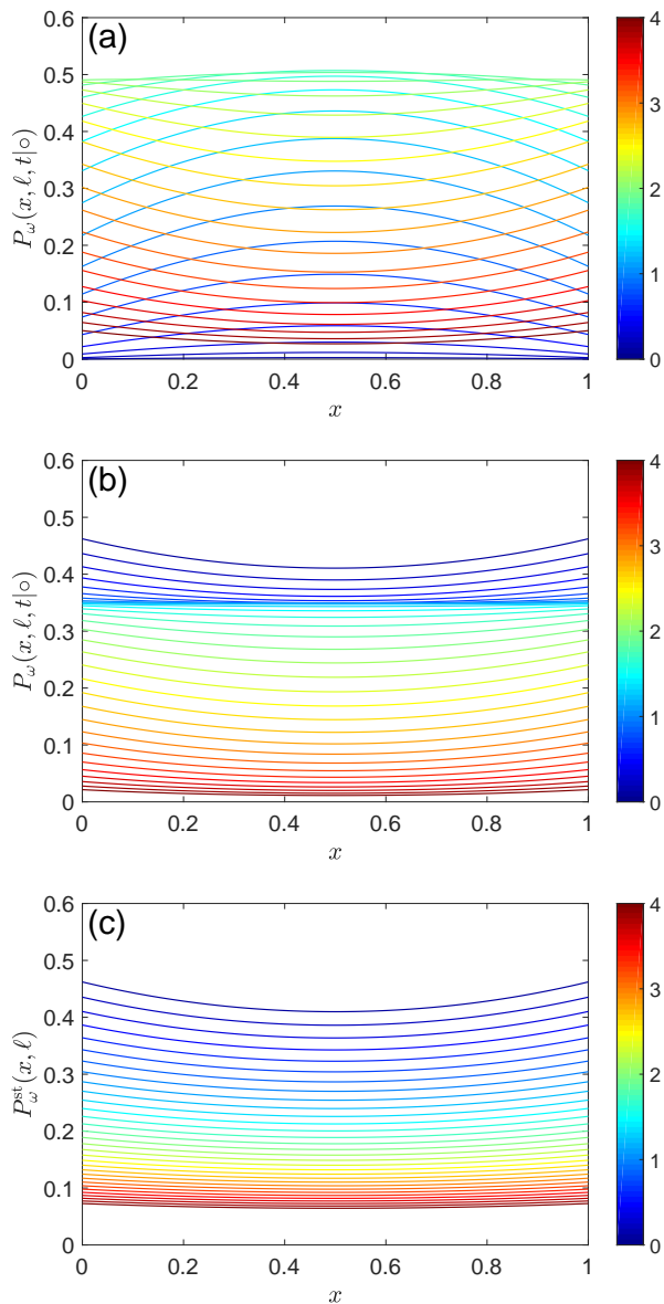
FIG. 7: The regular part of the volume-averaged full propagator P_\omega(x, \ell, t|o) under Poissonian resetting of the boundary local time at rate \omega for diffusion on the unit interval ( b = 1 ). It is plotted as a function x for multiple values of \ell , with D = 1 . Three panels correspond to t = 1 , \omega = 0 (a), t = 1 , \omega = 1 (b), and t = \infty , \omega = 1 (c). 33 colored curves correspond to 33 equally spaced values of \ell ranging from 0 (dark blue) to 4 (dark red).
