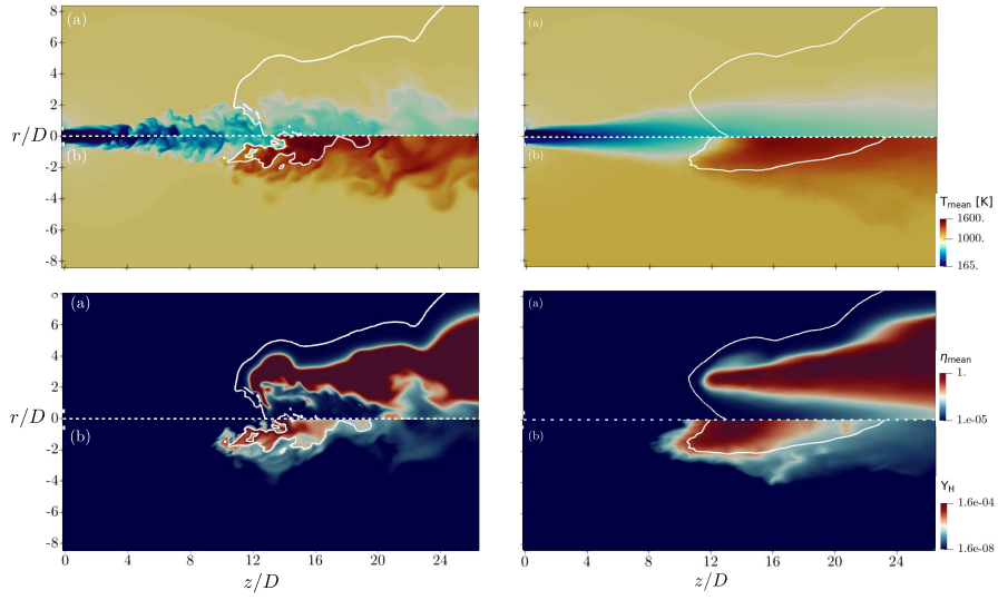
Fig. 41 Temperature (top) and \eta (bottom) contours for the cold flow simulation (a) compared to the reactive simulation (b). The auto-ignition condition ( \eta = Y_{\text{OH}}^0 / 1000 ) is indicated by white-line contours for non-reactive computations and for Y_{\text{OH}} = 6 \times 10^{-4} as taken from the reactive simulation [175]. Instantaneous quantities are represented in the left column, while mean quantities are in the right column.
