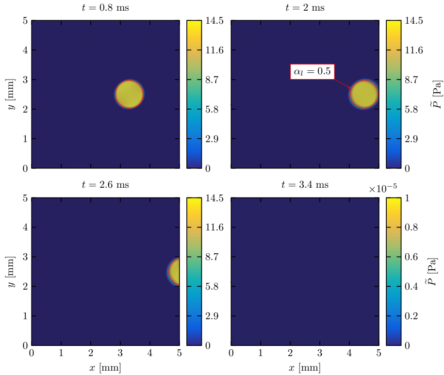
Figure 6: 2D liquid \text{H}_2\text{O} droplet advection to the outlet boundary condition with. \tilde{P} = P - P_0 . The red circle is \alpha_l = 0.5 isocontour. Note that the colorbar is rescaled for the last instant.
