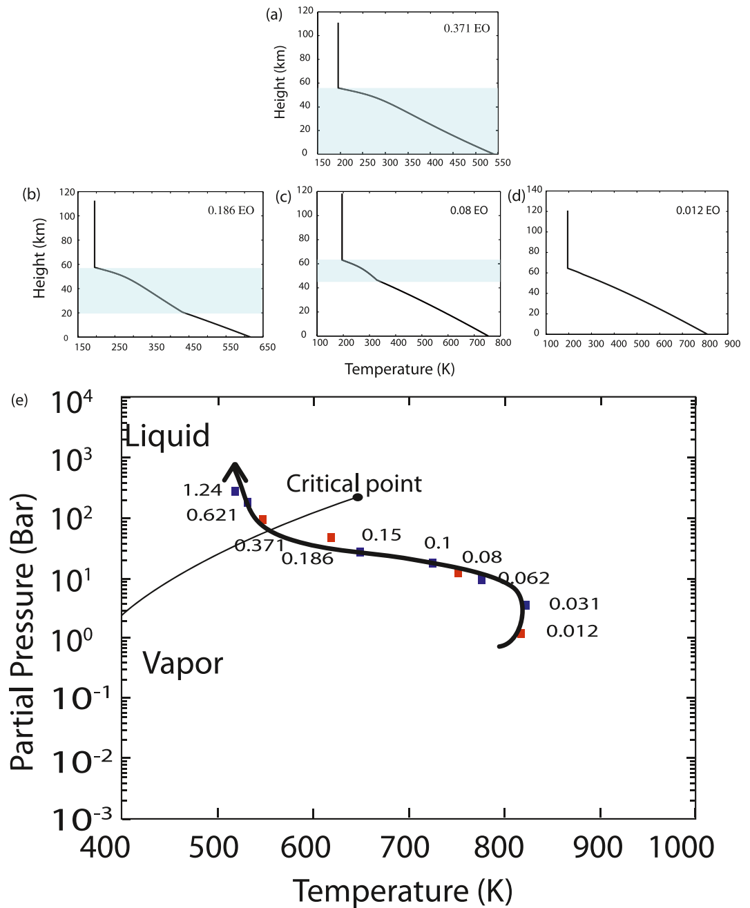
Figure 5. Water phase diagram and surface conditions at End of the Rapid Cooling Stage for an initial CO 2 content of 4 \times 10^{-2} wt% in the case of Earth ( D = 1 AU). The red squares on (e) indicate conditions for which we plot the atmospheric temperature profiles (a–d). The numbers on the thick black curve of (e) are the water contents initially dissolved in the Magma Ocean. The light blue zones drawn in the atmospheric profiles (a–d) show the part of the atmosphere where condensation occurs. For water content greater than 0.35 here, this zone extends to the surface to form a water ocean. See Massol et al. (2023b) for data.
