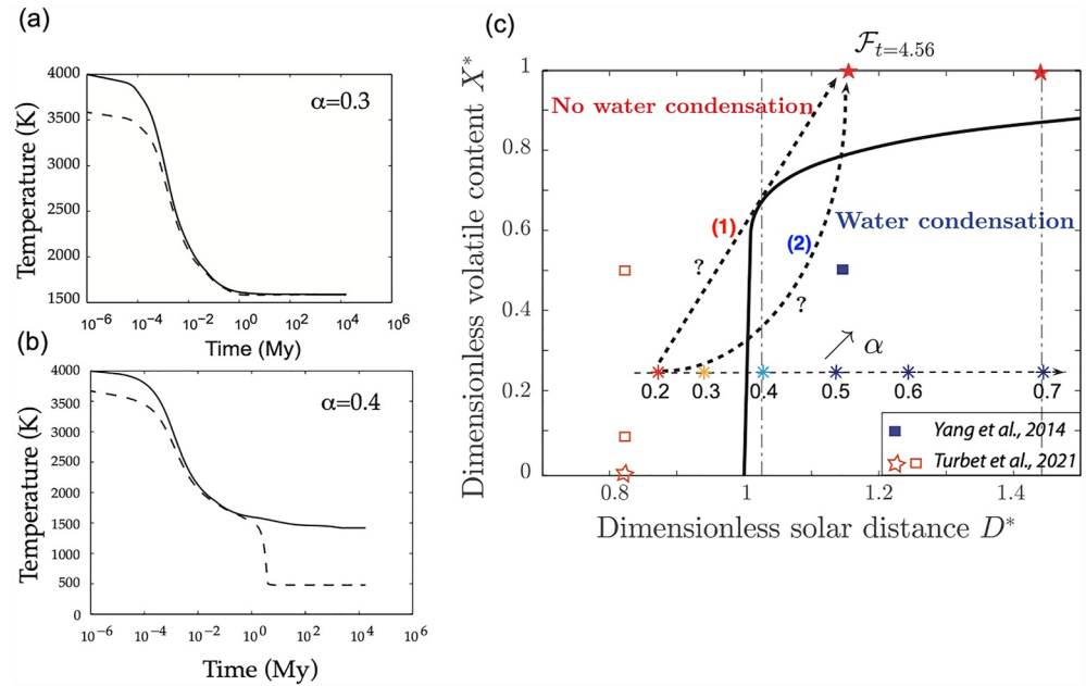
Figure 10. Scenarios for the early evolution of Venus. Dashed vertical lines represent D^* for albedo 0.4 and 0.7 for Venus and early solar constant. The intersection with the curve allows determination of the minimum amount of water necessary to condense at the surface. 3D models by Yang et al. (2014) and Turbet et al. (2021) are represented by filled blue square and empty red squares and star, respectively. Red-filled stars represent the present-day atmosphere of Venus with F_{t=4.56} standing for the present-day solar flux. See text for explanations about the dashed curves (1) and (2). See Massol et al. (2023b) for data.
