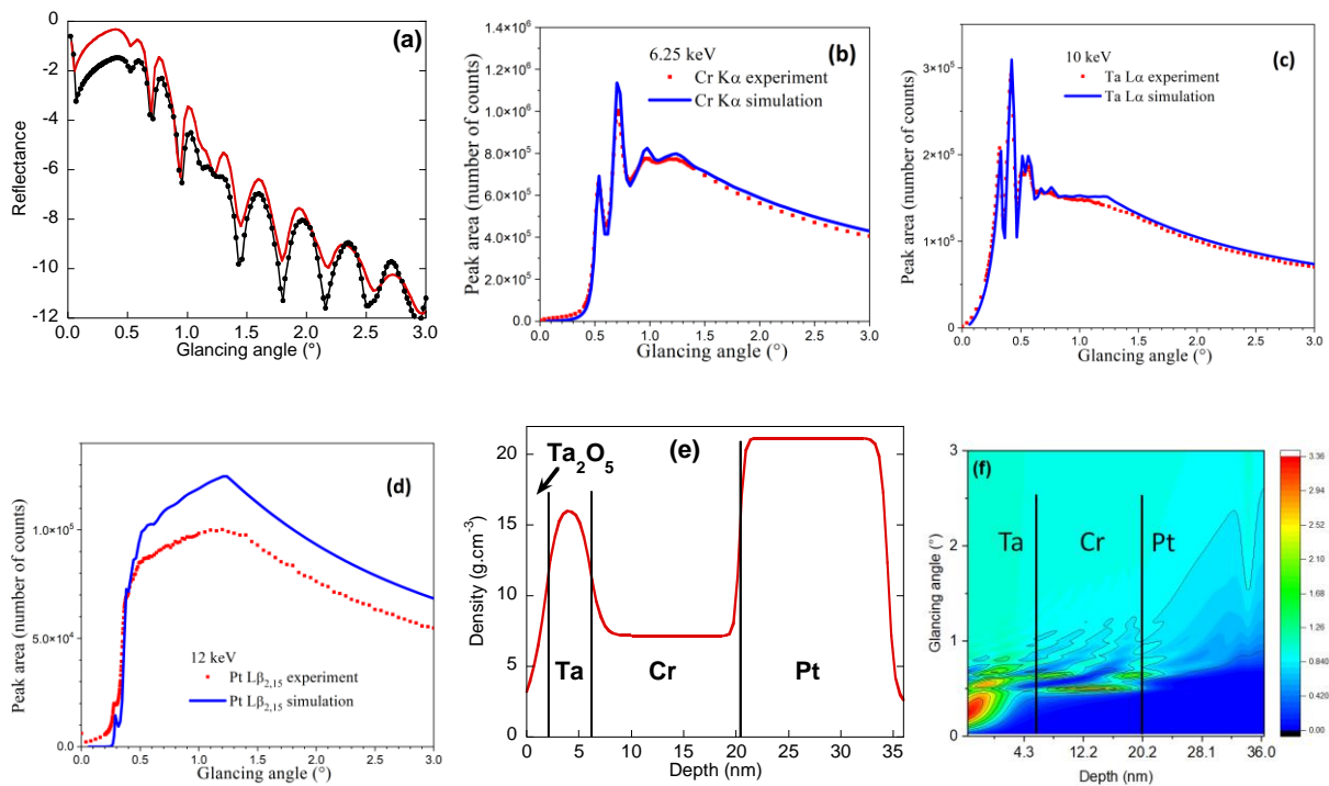
Figure 4: Simulations (lines) of the set of results (dots) of the sample “10 nm Cr” by a Ta_2O_5/Ta/Cr/Pt/PtSi/Si substrate model. (a) XRR curve (in log scale) at 6.25 keV; GIXRF curves (in linear scale) of (b) Cr at 6.25 keV, (c) Ta at 10 keV and (d) Pt at 12 keV; (e); variation of the density of the stack
