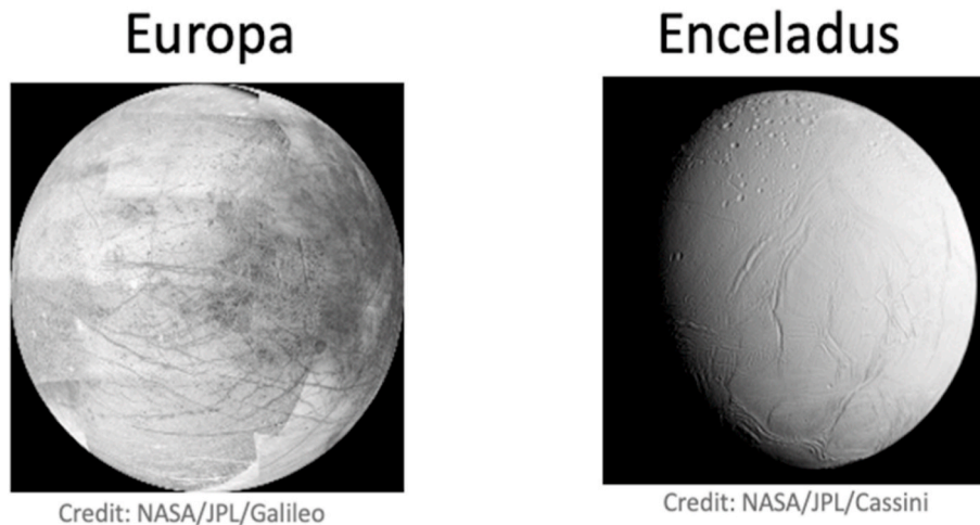
Fig. 3. New Policy considerations were implemented for icy moons, like Jupiter's moon Europa and Saturn's moon Enceladus.
