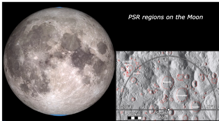
Fig. 2. Right side, red features: PSRs at the Moon's south pole are further protected in the new Policy. Left side: fine blue caps concentrated at the poles are also protected while other regions have relaxed requirements. Credit: LRO/NASA. (For interpretation of the references to colour in this figure legend, the reader is referred to the Web version of this article.)
