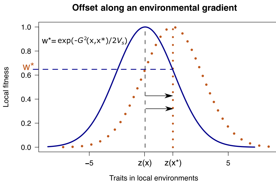
FIG. 1. Geometric offset (genetic gap) under local Gaussian stabilizing selection. The two points, z(\mathbf{x}) = \bar{z} and z(\mathbf{x}^*) = \bar{z}^* , represent locally optimal values of an adaptive trait in respective environments \mathbf{x} and \mathbf{x}^* . The curves display the fitness values for the trait in each environment. An organism with trait z(\mathbf{x}) , optimal in environment \mathbf{x} , being placed in altered environment \mathbf{x}^* , has a fitness value equal to \omega^* = \exp(-G^2(\mathbf{x}, \mathbf{x}^*)/2V_s) , where G^2(\mathbf{x}, \mathbf{x}^*) is the genomic offset (horizontal dashed line), and V_s is defined in text.
