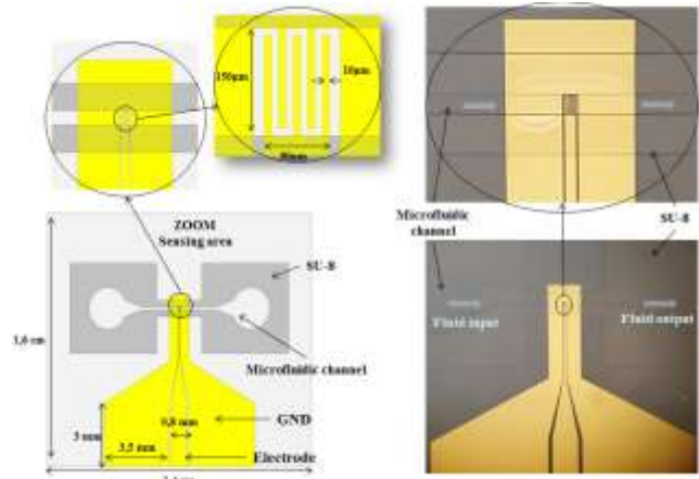
Fig. 2. Interdigitated capacitor structure in top view (left simulated and (right) fabricated.
