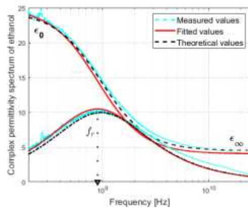
Fig. 13. Real and imaginary parts of the dielectric permittivity of ethanol fitted or extracted from the measurement using the calibration media (air, deionized water, methanol).
