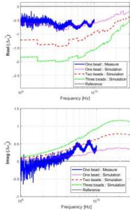
Fig. 16. Real and imaginary parts of the difference between water permittivity and the ones extracted from measurement with one polystyrene particle or simulations with one, two or three particles on the IDC.
