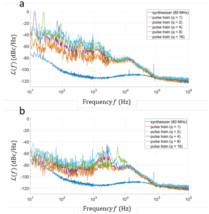
Fig. 11. a (resp. b): phase noise in different Talbot conditions without (resp. with) feedback. The error signal comes from the relative phase between a reference RF signal and the first harmonic of the pulse train intensity.
