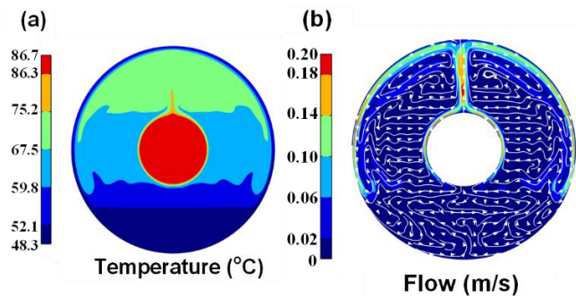
Fig. 7. The distribution of the temperature and convection in 550kV GIL at 5.6 kA. (a) The temperature distribution. (b) The convection distribution, and arrows indicate flow directions.
