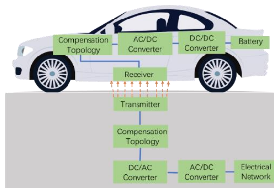
Fig.1. An inductive power transfer system
