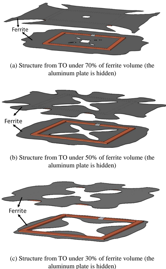
Fig.8. Ferrite placement with an aluminum plate
