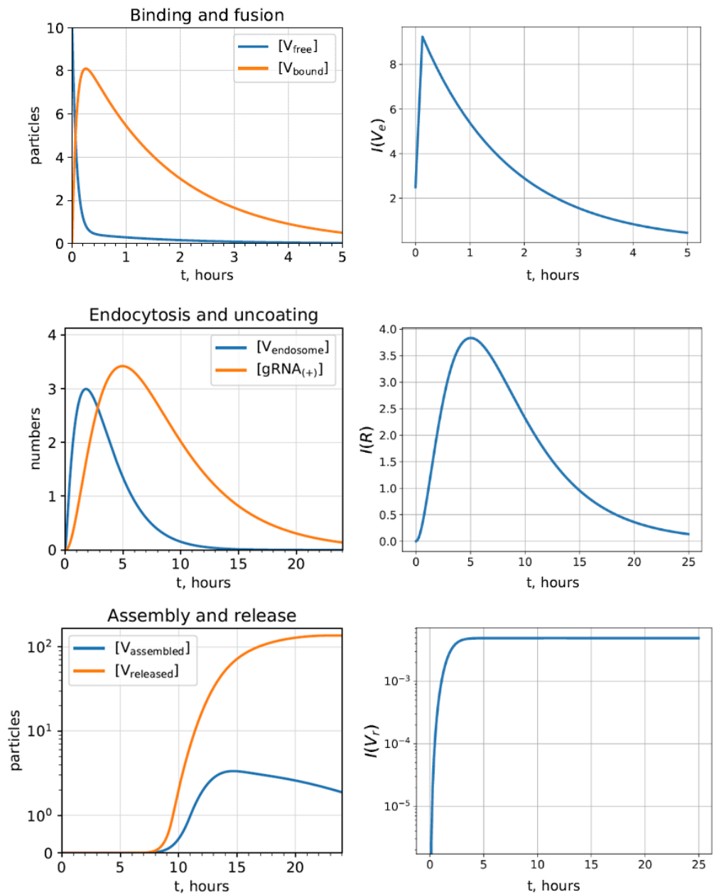
Figure 5. Comparison of the kinetics of SARS-CoV-2 replication predicted by model (1)–(5) (right) with results from ([21], Figure 2) (left). The values of parameters are estimated from the model reduction (Table 1): k_1 = 0.5 , q_1 = 0.5 , \sigma_1 = 0.12 , \sigma_2 = 0.2 , k_3 = 0.003 , q_2 = 0 , k_4 = 6.093 , and the initial conditions are V_e(0) = 1 , A(0) = 1 , V_i(0) = 0 , R(0) = 0 , V_r(0) = 0 . From top to bottom: [V_{free}] corresponds to V_e , [gRNA_{(+)}] corresponds to R , and [V_{assembled}] corresponds to V_r . The difference in maximal values of [V_{assembled}] and V_r is explained by biases due to numerous transformation of the parameters required for reduction in obtaining coefficient k_3 , which influences the amplitude of V_r accordingly (78), and the absence of a decrease in the end part of the plot is explained by the fact that there is no mortality in the model (1)–(5) for V_r (and q_2 = 0 for these calculations).
