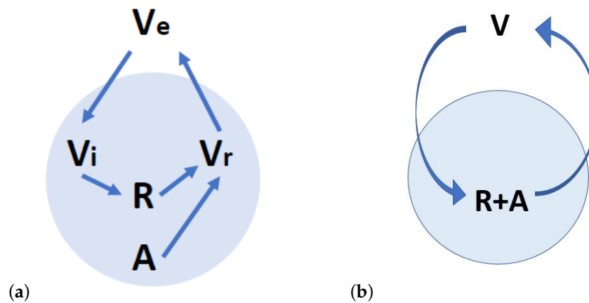
Figure 1. Basic model considered in this work (a) with extracellular virus V_e , intracellular virus V_i , viral genetic material R , and intracellular proteins A participating in virus replication and production of new virus particles V_r . In the reduced model (b), two intermediate stages are omitted.
