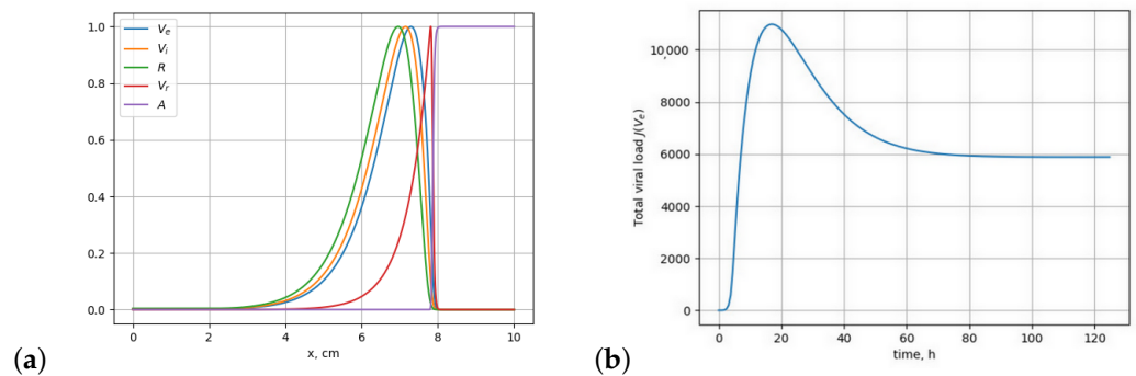
Figure 2. Numerical simulations of system (1)–(5). (a) Concentration profiles as functions of space; (b) viral load as a function of time. The values of parameters are as follows: D_1 = 0.001 \text{ cm}^2 \text{ h}^{-1} , k_1 = 0.5 \text{ h}^{-1} , q_1 = 0.09 \text{ h}^{-1} , \sigma_1 = 0.01 \text{ h}^{-1} , k_3 = 1000 \text{ mL} (\text{h} \times \text{unit})^{-1} , q_2 = 0.1 \text{ h}^{-1} , \sigma_2 = 0.36 \text{ h}^{-1} , k_4 = 0.4 \text{ mL} (\text{h} \times \text{copy})^{-1} ; Initial conditions: V_e(0) = 1 \text{ copy/mL} , A = 4 \text{ unit/mL} , V_i = V_r = R = 0 . Normalization (for the left plots): \max(V_e) = 3619.4 ; \max(V_i) = 635.8 ; \max(R) = 845.7 ; \max(V_r) = 8863.8 ; \max(A) = 4 .
