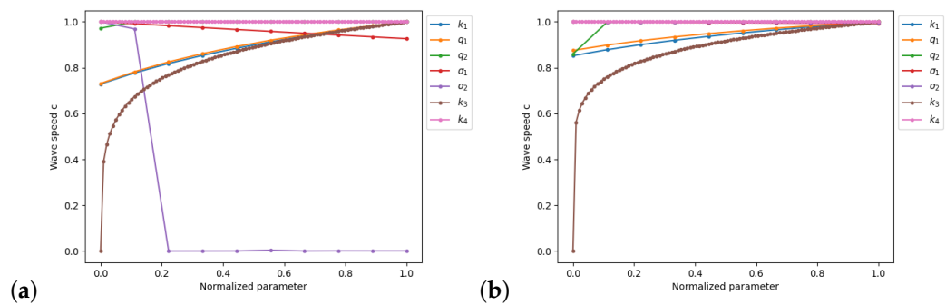
Figure 4. The dependence of the wave speed in the system (1)–(5) on parameters. (a) All the parameters are in their estimated ranges from Table 1, and the ranges are projected to the [0, 1] interval by a linear function. Fixed parameters are the same as listed in Figure 3. (b) Different values for the fixed parameters (from Table 1); the results for q_1 correspond to Figure 3b.
