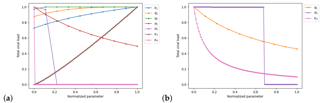
Figure 3. The dependence of the total viral load in the system (1)–(5) on parameters. (a) All the parameters are in their estimated ranges from Table 1, and the ranges are projected to the [0, 1] interval by a linear function. For each varying parameter, the other ones are fixed using the following values: k_1 = 0.055 , q_1 = 0.1 , \sigma_1 = 3 , \sigma_2 = 0.08 , k_3 = 100 , q_2 = 8 , k_4 = 0.1 , D = 0.01 , A_0 = 1 , L = 10 cm. Units of the parameters are the same as in Figure 2. (b) The parameter k_4 is in the range [1.9 \times 10^{-5}, 1.9 \times 10^{-4}] , and parameter \sigma_2 is in range [0.129, 0.131] . These are the ranges corresponding to the straight lines for these parameters on the left figure. The dependence for the parameter q_1 is represented for the other set of fixed parameters (values from Table 1).
