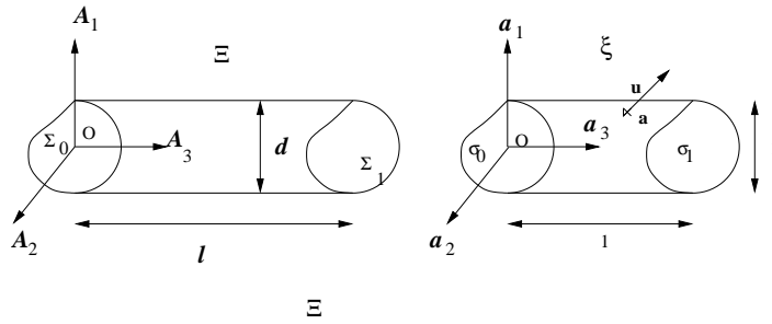
Figure 1: the beam
