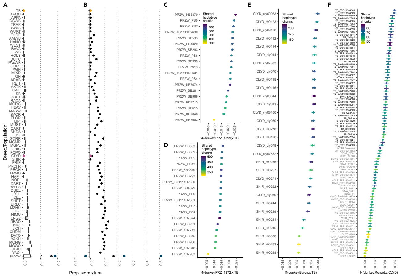
Figure 3. Przewalski Horse (PH) admixture and relationship between modern and ancient horses
