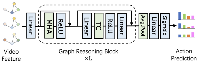
Figure 5: Graph Classification.
