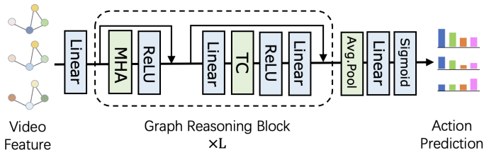
Figure 5: Graph Classification.
