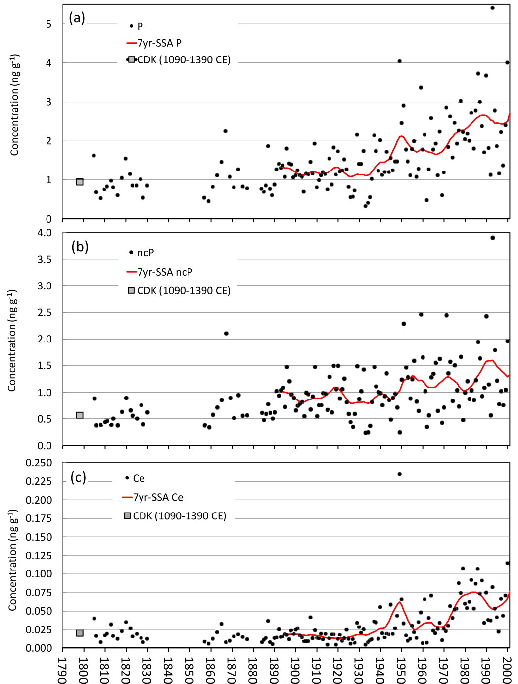
Figure 3. Long-term Col du Dôme ice-core trend in summer of P (a), non-crustal P (b), and Ce (c) (not corrected from the under-recovery, Section 2.1). The gray squares on the left are values observed in CDK ice (1090–1390 common Era, see Section 2.1 and Table 2). The red lines are first component of singular spectrum analysis with a 7-year time window. Note the large Ce value observed in 1949 (0.234 ng g -1 ).
