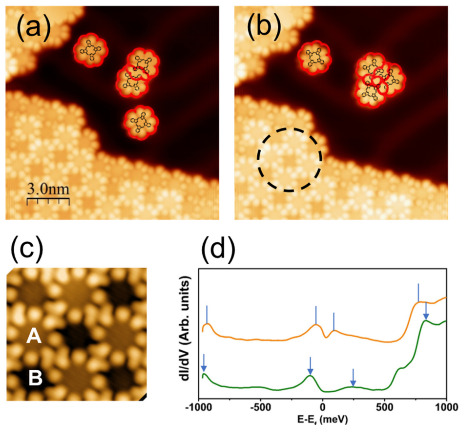
Figure 2. (a,b) Constant current STM images (70 pA, -0.3 V) of TbPc 2 molecular islands and clusters grown on Au(111). Contours of upper Pc's are highlighted in red. (c) Zoom-in image of the circled area in (b) showing bright (A) and dark (B) contrasts for molecules in a domain (70 pA, -0.3 V). (d) dI/dV spectroscopy performed at the center of A-type (orange) and B-type (green) molecules, respectively. Vertical lines/arrows show the correspondence between different peaks. (a,b) from ref [6] with permission. Further permissions related to the material excerpted should be directed to the ACS.
