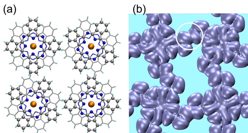
Figure 3. (a) Primitive cell 1 \times 1 of an assembly of four TbPc 2 molecules with periodic boundary conditions. Balls: upper Pc; sticks: lower Pc. Color code: C (grey), N (blue), Tb (orange). The only experimental input is the dimension of the square lattice (1.42 nm). After full relaxation, it is found that the dihedral angle \theta = 45^\circ for all the molecules and remains unchanged independent of initial configuration. (b) Electron density 1 \times 10^{-5} \text{ e}/\text{\AA}^3 in the range [E_F - 0.6 \text{ eV}, E_F] , top view, above the upper Pc. The circle indicates the molecular orbital overlap between adjacent molecules.
