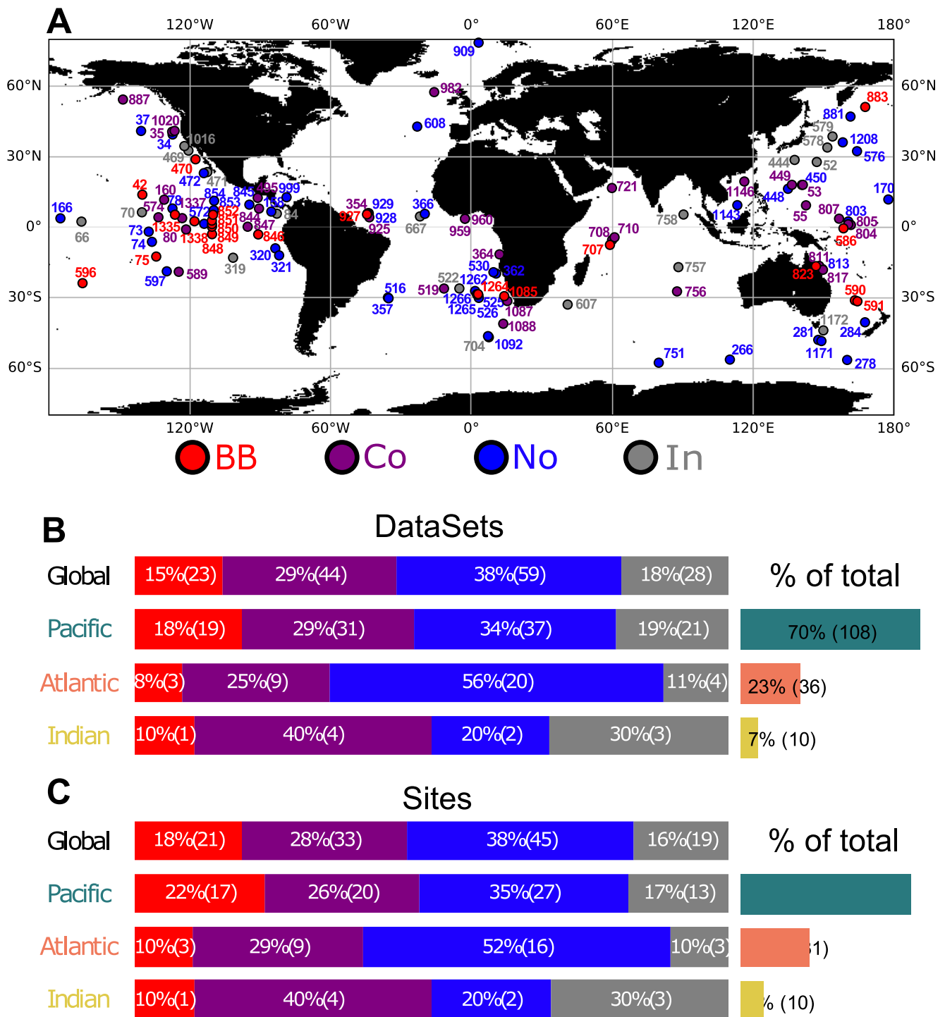
Figure 2. (a) Present-day coastlines with dots showing the modern positions of the 118 labeled sites. (b) Distribution of labels for the 154 data sets, with the absolute value in brackets. (c) Distribution of labels for the 118 sites, with the absolute value in brackets. “In”—Inconclusive; “No”—No LMBB; “Co”—Controversial LMBB; and “BB”—LMBB is present.
