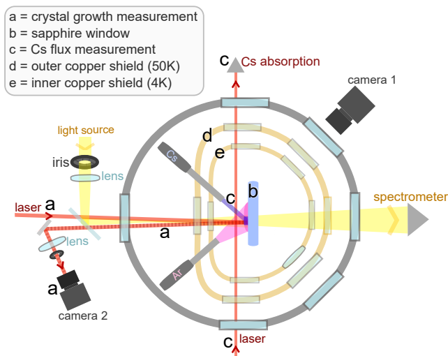
FIG. 1. (Color available online) Schematic representation of the cryostat and the optical systems utilized to monitor the matrix growth rate and to measure the absorption and fluorescence spectra. The arrows indicate the propagation directions of the beams. The laser illumination of the matrix is imaged on CCD camera 2 to display the interference pattern.
