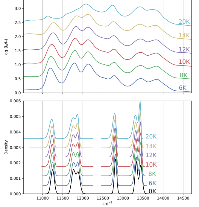
FIG. 9. Comparison of observed absorption with the simulated one using the temperature scaled first order crystal fields model. The model incorporates the modified reflection approximation (Eq. (12)), using parameters from Table II. The theoretical spectra are generated from a density kernel estimation of the Monte Carlo simulation results. Results for the T_d and O_h sites are shifted in energy by a global offset for easier comparison with the experimental data (that are 1650 \text{ cm}^{-1} and 85 \text{ cm}^{-1} respectively for O_h and T_d ). Vertical offsets have been applied to both experimental and theoretical spectra to enhance visual clarity.
