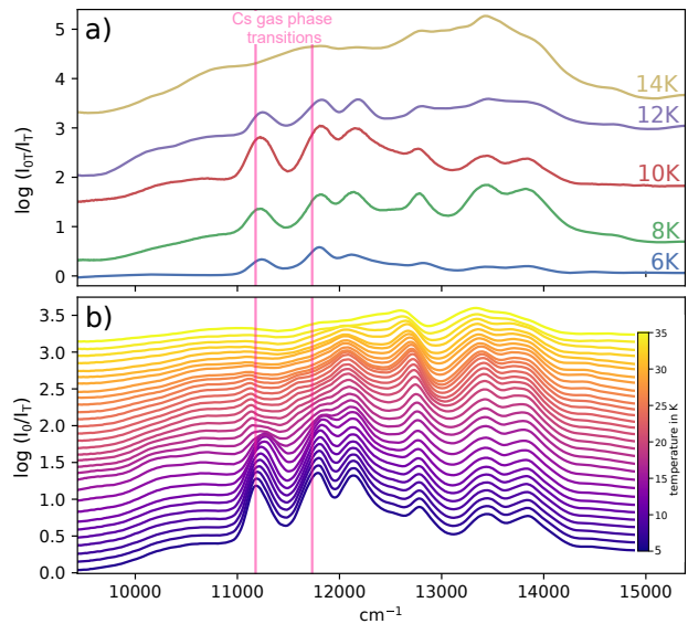
FIG. 2. a) Absorbance spectra of Cs embedded in Ar for deposits conducted at different temperatures. b) Evolution with temperature for a spectrum initially created at 8 K. The spectra are offset in ordinate for better visual clarity. The positions of the 6s_{1/2} \rightarrow 6p_{1/2} (left) and 6s_{1/2} \rightarrow 6p_{3/2} (right) Cs gas-phase transitions are indicated for reference.
