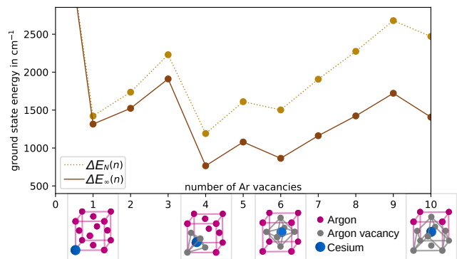
FIG. 4. For a given number of vacancies n , the optimized configuration found to lower \Delta E(n) is displayed (calculation performed with N = 1372 atoms). The figure illustrates both \Delta E(n) and \Delta E^\infty(n) , alongside a depiction of the final structure realized for the Cs atom and a few of the nearest-neighbor Ar atoms.
