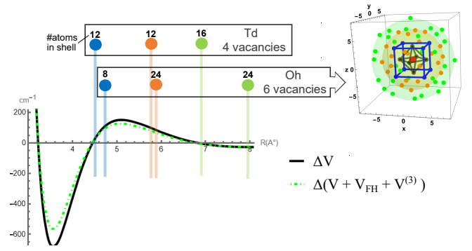
FIG. 6. This figure illustrates \Delta V = 2V_{\Pi} + V_{\Sigma} - V_X Cs-Ar potentials with an offset of the asymptotic values. The first R_1 , second R_2 , and third R_3 nearest neighbor shells in the T_d and O_h scenarios are provided (for the O_h case, an example of the Cs and Ar positions is also given).
