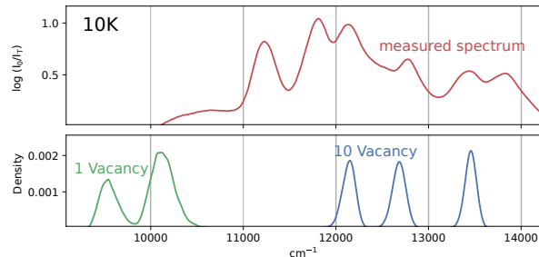
FIG. 7. Comparison between the experimental absorption spectrum and theoretical semi-classical Mulliken formula (4) for the 1 and 10 vacancy sites at 10 K.
