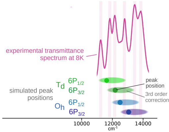
FIG. 5. This figure presents a comparison between an experimental transmittance spectrum (represented by the solid pink lines), for the two trapping sites, O_h with 6 vacancies, and T_d with 4 vacancies. The lower section indicates the position of the 0 K lines employing pairwise potential, where dots correspond to the two-body cases with potentials sourced from [42]. The influence of zero point energy on these lines is marginal (at most 150 \text{ cm}^{-1} ). However, the incorporation of the third-order effect (refer to the main text) results in an additional shift that we predict to fall within the elliptical regions.
