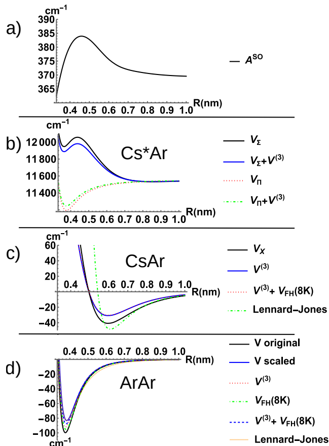
FIG. 3. a) Spin-orbit constant for Cs(6p)-Ar interaction. b) Cs(6p)-Ar potential curves. c) Cs(6s)-Ar potential curves. d) Ar-Ar ground state potential curves. The potential curves V used in this study are compared to the zero-point energy V_{FH} , and a third-order correction V^{(3)} . The original potentials are taken from [42]. For the excited state, we chose to plot only a third-order case with no cut-off (in analogy with the ground state case, see text); i.e., the two-body potential V (offset by E(6p) ) multiplied by \frac{1}{3} \frac{8\pi\rho}{9} \frac{C_9^*}{C_6^*} .
