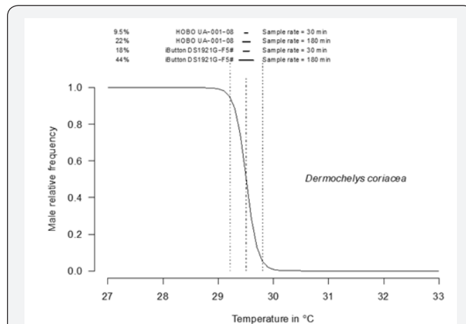
Figure 3: Pattern of temperature-dependent sex determination in the marine turtle Dermochelys coriacea (Chevalier et al. 1999). The pivotal temperature is 29.52°C and the range of transitional range of temperatures (TRT) is 0.59°C. At the top, the uncertainty of average 10days of temperatures is shown for various situations. The percentages indicate the relative proportion of the TRT as compared to the uncertainty of the 10 days average temperatures.
