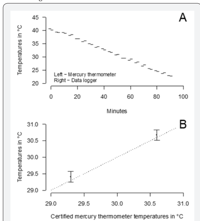
Figure 2: A. Temperature recorded with certified mercury thermometer, and data logger. B. Recorded temperatures with data logger calibrated using mercury thermometer temperatures from A.
