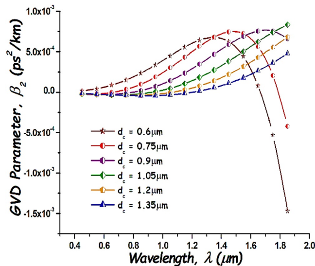
Figure 18. Group-velocity dispersion of flower-cladding photonic crystal fiber for various core diameters.
