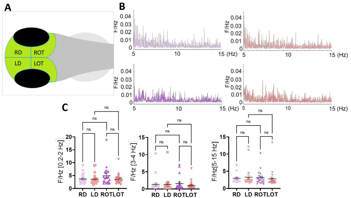
Fig. 5. Brain voltage patterns in four brain regions of interest. A: Cartoon showing the four regions of interest (ROIs) that we selected in the brain, the right diencephalon (RD), left diencephalon (LD), right optic tectum (ROT), and left optic tectum (LOT). B: Example of FT of brain voltage activity for 5–15 Hz interval: RD (clear purple), LD (clear red), ROT (dark purple), LOT (dark red). C: Quantifications of the brain voltage activities for the intervals 0.2–2, 3–4, and 5–15 Hz in control zebrafish larvae not treated with any contaminant (n = 21). Kruskal–Wallis test; *** p < 0.001, **** p < 0.0001. (For interpretation of the references to color in this figure legend, the reader is referred to the web version of this article).
